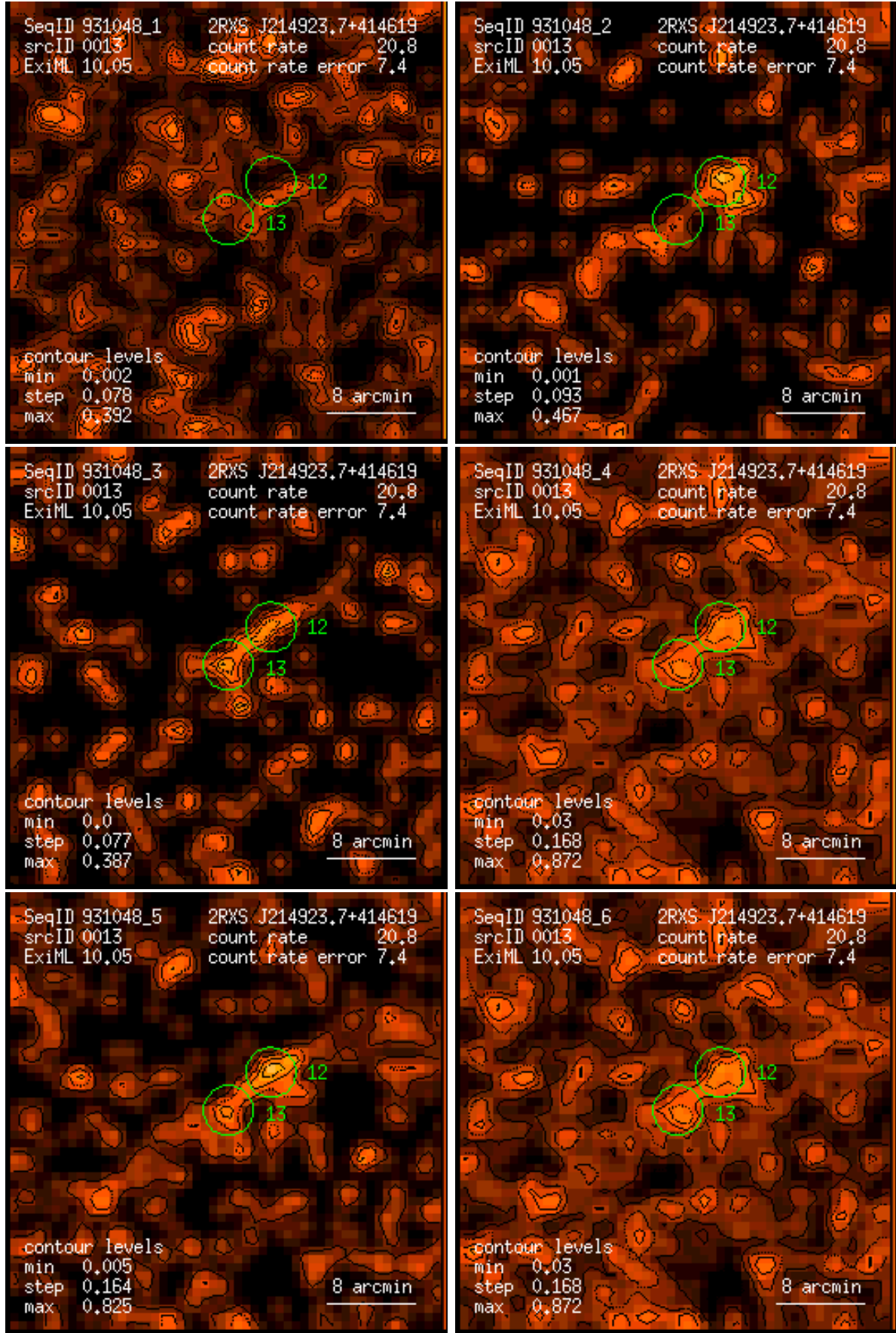
Figure 13: RASS 931048: detection 0013: band rate images, Gaussian filter: (1) PSPC channels 11 – 41, (2) 52 – 90, (3) 91 – 201, (4) 11 – 235, (5) 52 – 201, (6) 11 – 201. Broad band rates in counts/ks. Band rate contour levels in counts/ks/arcmin 2 .
