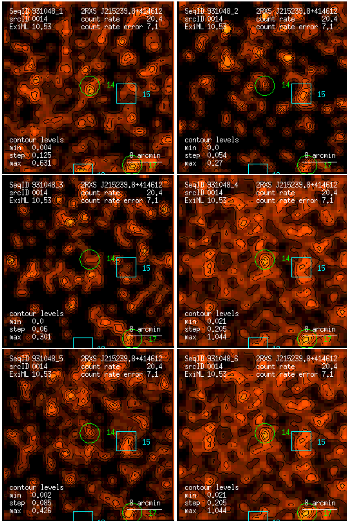
Figure 14: RASS 931048: detection 0014: band rate images, Gaussian filter: (1) PSPC channels 11 – 41, (2) 52 – 90, (3) 91 – 201, (4) 11 – 235, (5) 52 – 201, (6) 11 – 201. Broad band rates in counts/ks. Band rate contour levels in counts/ks/arcmin 2 .
