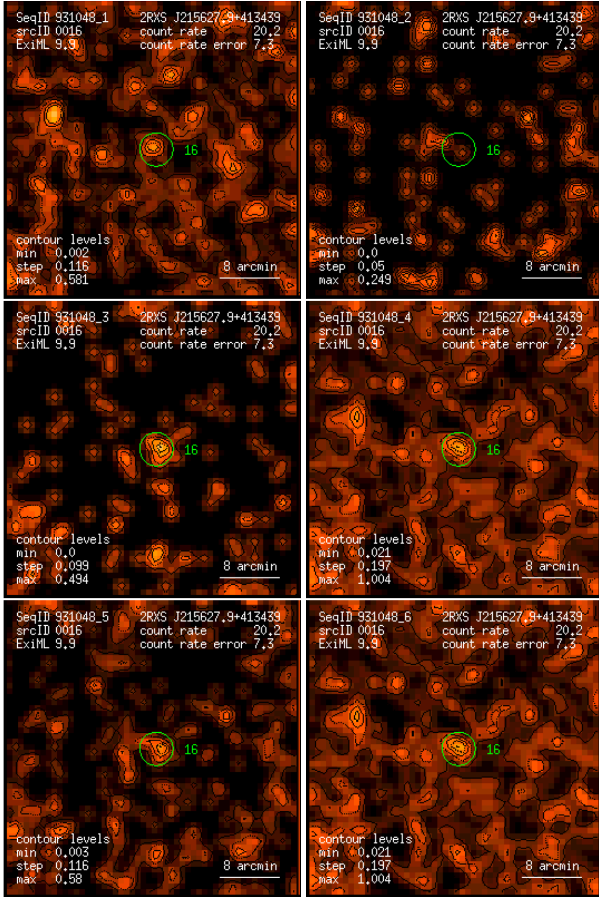
Figure 16: RASS 931048: detection 0016: band rate images, Gaussian filter: (1) PSPC channels 11 – 41, (2) 52 – 90, (3) 91 – 201, (4) 11 – 235, (5) 52 – 201, (6) 11 – 201. Broad band rates in counts/ks. Band rate contour levels in counts/ks/arcmin 2 .
