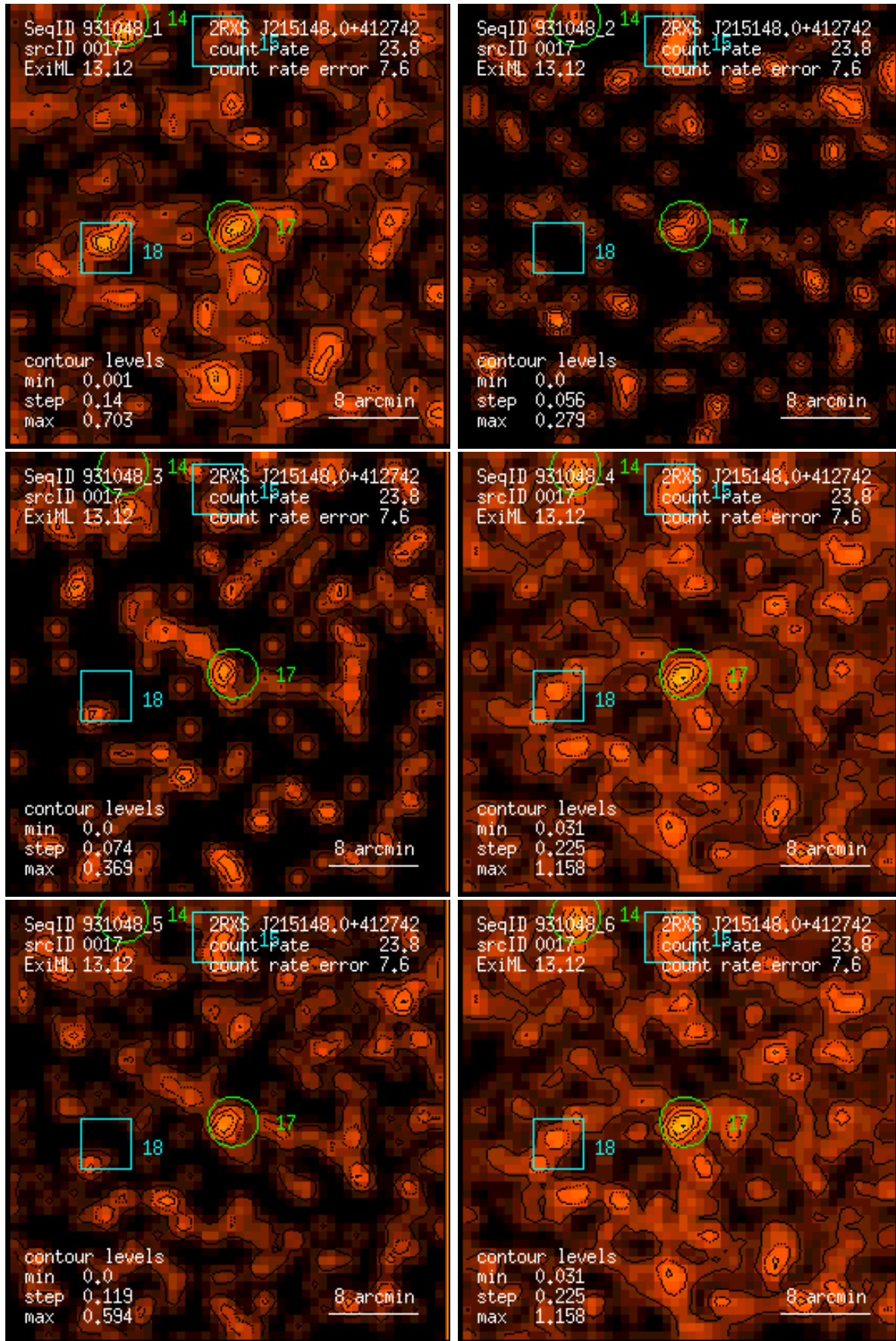
Figure 17: RASS 931048: detection 0017: band rate images, Gaussian filter: (1) PSPC channels 11 – 41, (2) 52 – 90, (3) 91 – 201, (4) 11 – 235, (5) 52 – 201, (6) 11 – 201. Broad band rates in counts/ks. Band rate contour levels in counts/ks/arcmin 2 .
