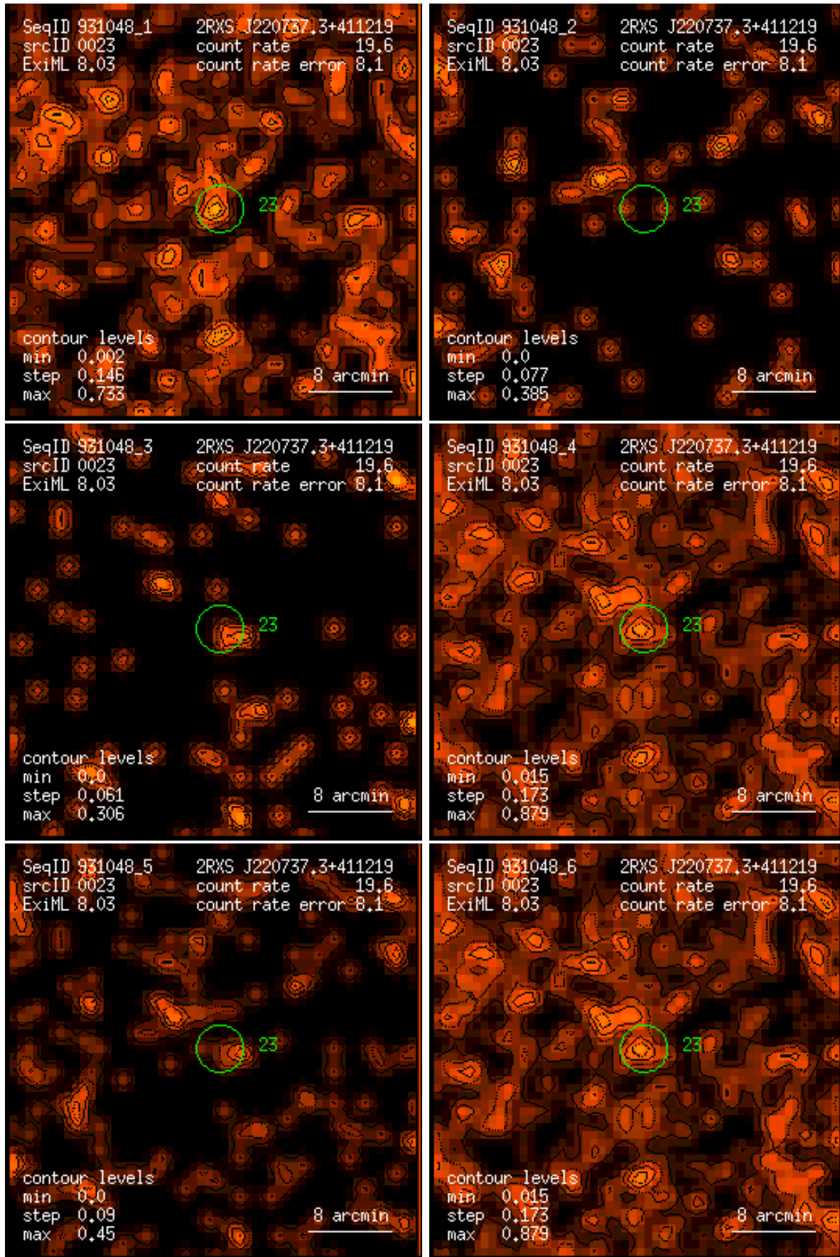
Figure 23: RASS 931048: detection 0023: band rate images, Gaussian filter: (1) PSPC channels 11 – 41, (2) 52 – 90, (3) 91 – 201, (4) 11 – 235, (5) 52 – 201, (6) 11 – 201. Broad band rates in counts/ks. Band rate contour levels in counts/ks/arcmin 2 .
