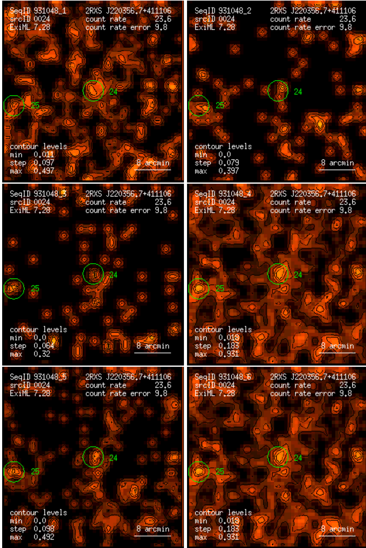
Figure 24: RASS 931048: detection 0024: band rate images, Gaussian filter: (1) PSPC channels 11 – 41, (2) 52 – 90, (3) 91 – 201, (4) 11 – 235, (5) 52 – 201, (6) 11 – 201. Broad band rates in counts/ks. Band rate contour levels in counts/ks/arcmin 2 .
