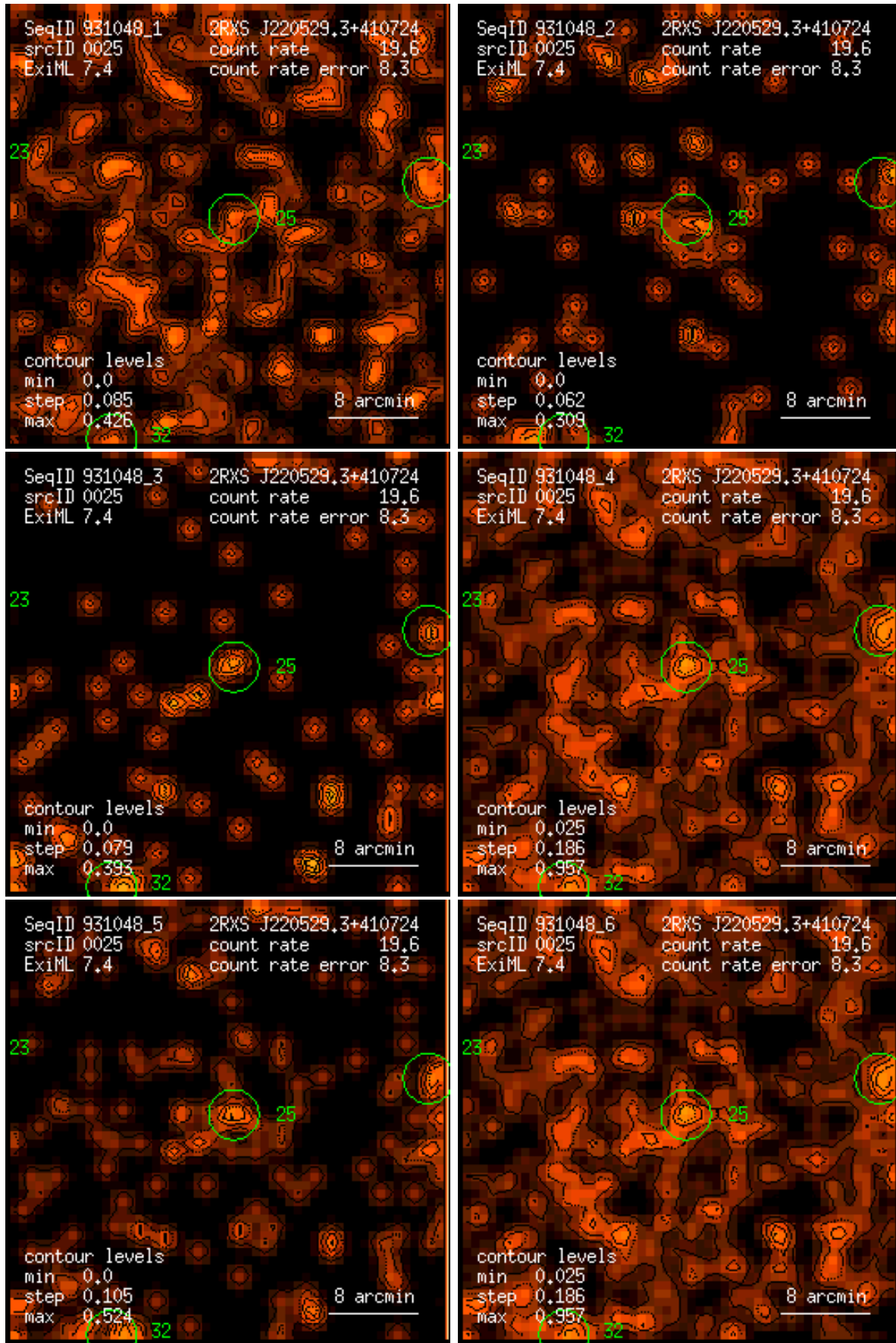
Figure 25: RASS 931048: detection 0025: band rate images, Gaussian filter: (1) PSPC channels 11 – 41, (2) 52 – 90, (3) 91 – 201, (4) 11 – 235, (5) 52 – 201, (6) 11 – 201. Broad band rates in counts/ks. Band rate contour levels in counts/ks/arcmin 2 .
