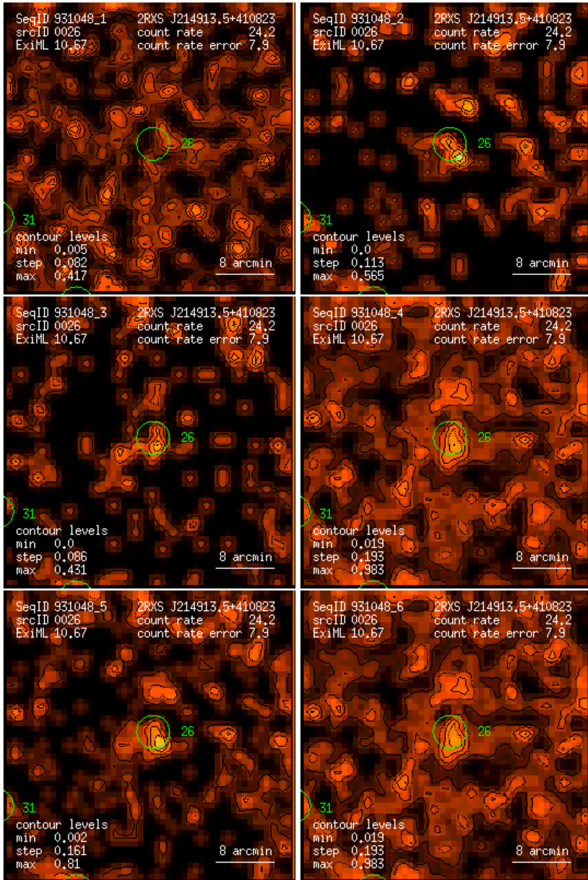
Figure 26: RASS 931048: detection 0026: band rate images, Gaussian filter: (1) PSPC channels 11 – 41, (2) 52 – 90, (3) 91 – 201, (4) 11 – 235, (5) 52 – 201, (6) 11 – 201. Broad band rates in counts/ks. Band rate contour levels in counts/ks/arcmin 2 .
