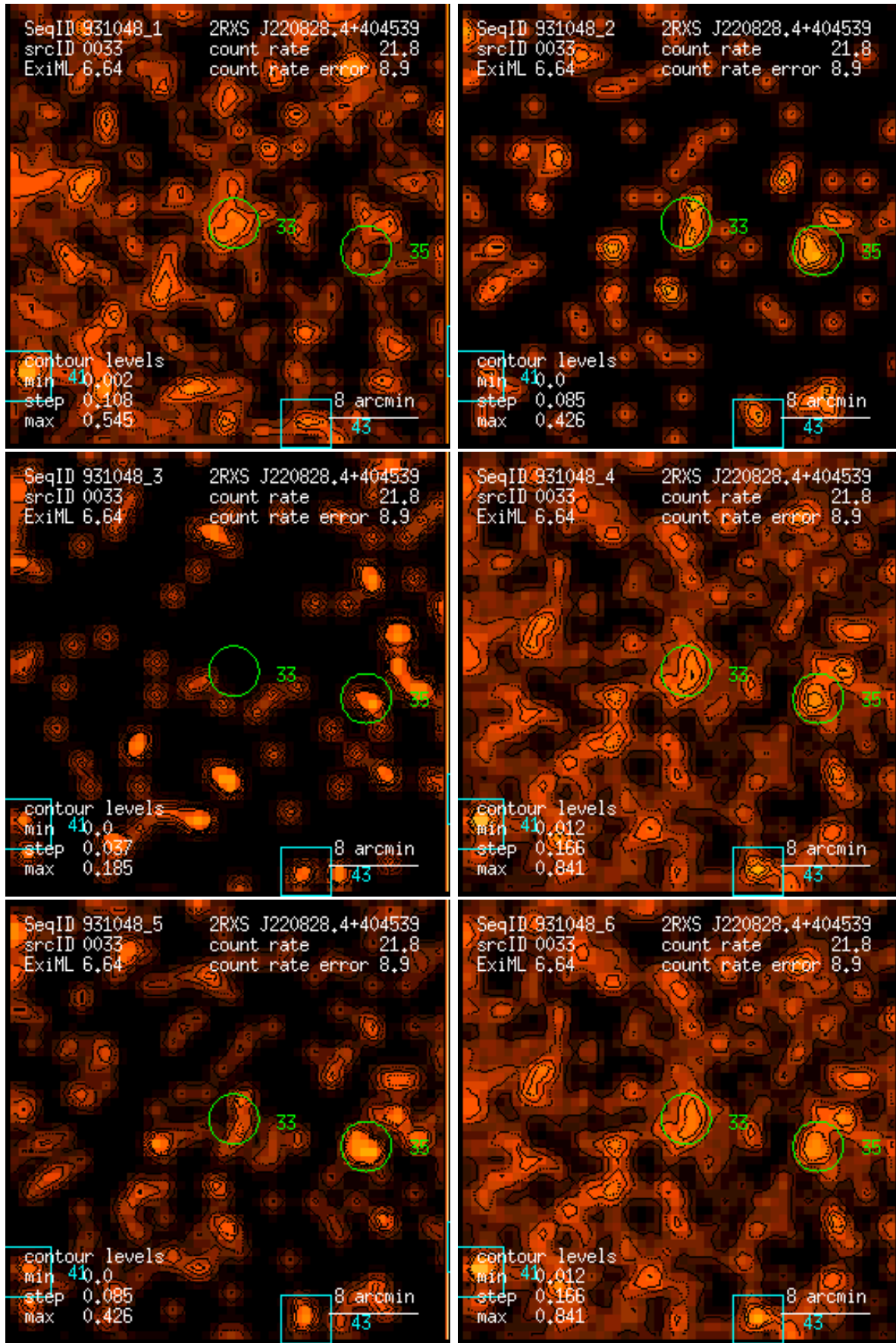
Figure 33: RASS 931048: detection 0033: band rate images, Gaussian filter: (1) PSPC channels 11 – 41, (2) 52 – 90, (3) 91 – 201, (4) 11 – 235, (5) 52 – 201, (6) 11 – 201. Broad band rates in counts/ks. Band rate contour levels in counts/ks/arcmin 2 .
