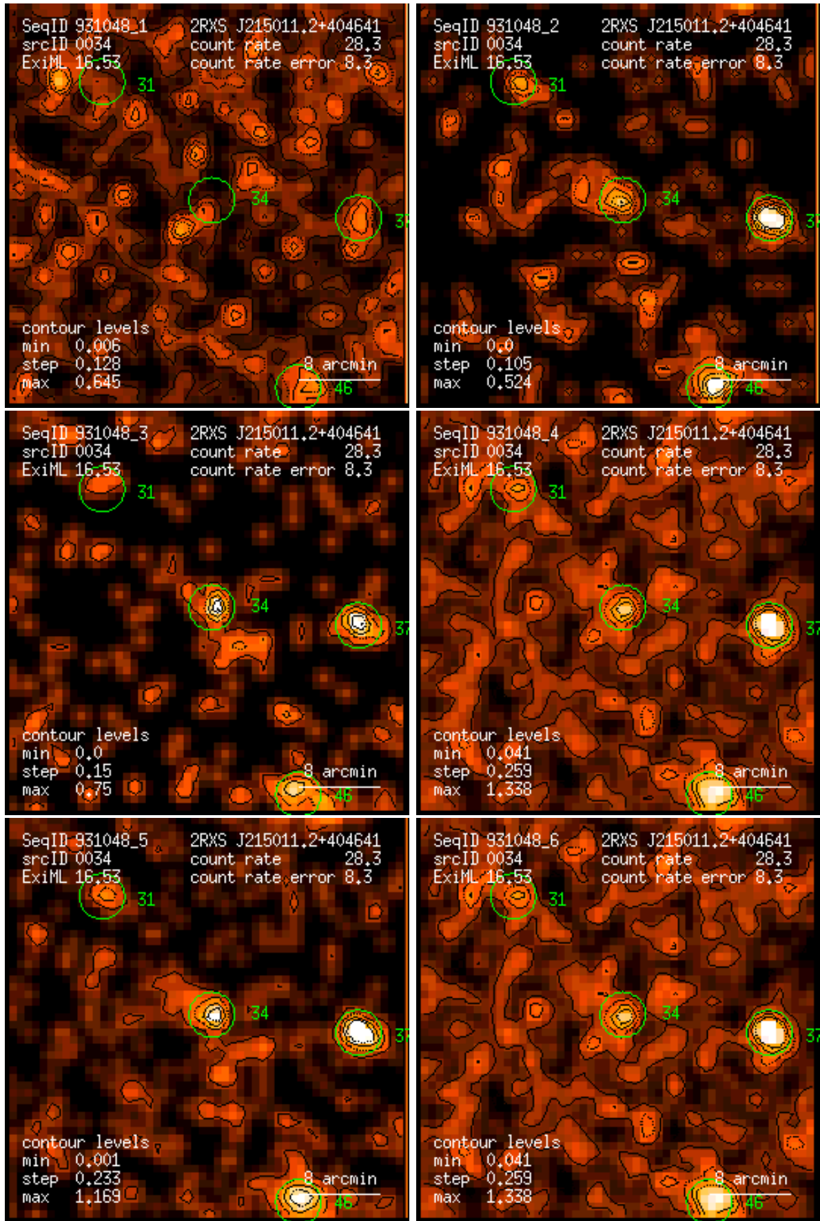
Figure 34: RASS 931048: detection 0034: band rate images, Gaussian filter: (1) PSPC channels 11 – 41, (2) 52 – 90, (3) 91 – 201, (4) 11 – 235, (5) 52 – 201, (6) 11 – 201. Broad band rates in counts/ks. Band rate contour levels in counts/ks/arcmin 2 .
