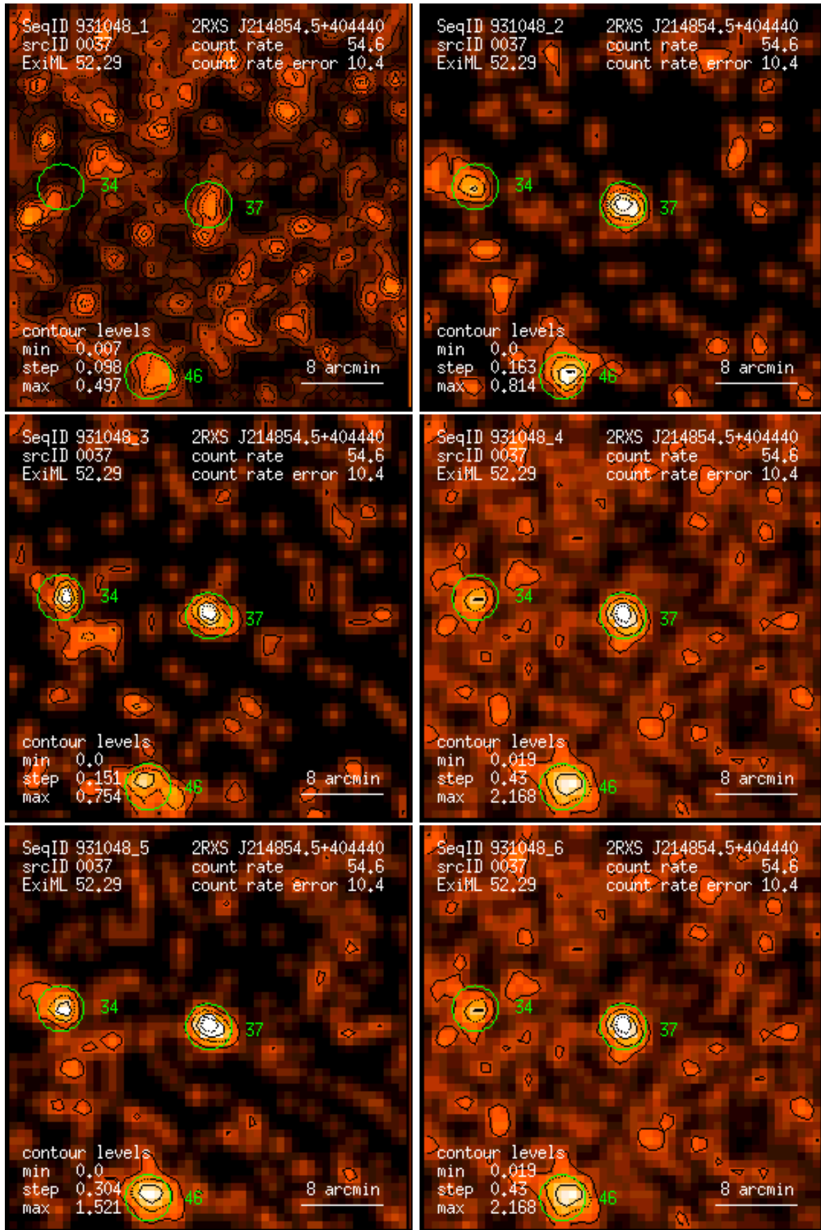
Figure 37: RASS 931048: detection 0037: band rate images, Gaussian filter: (1) PSPC channels 11 – 41, (2) 52 – 90, (3) 91 – 201, (4) 11 – 235, (5) 52 – 201, (6) 11 – 201. Broad band rates in counts/ks. Band rate contour levels in counts/ks/arcmin 2 .
