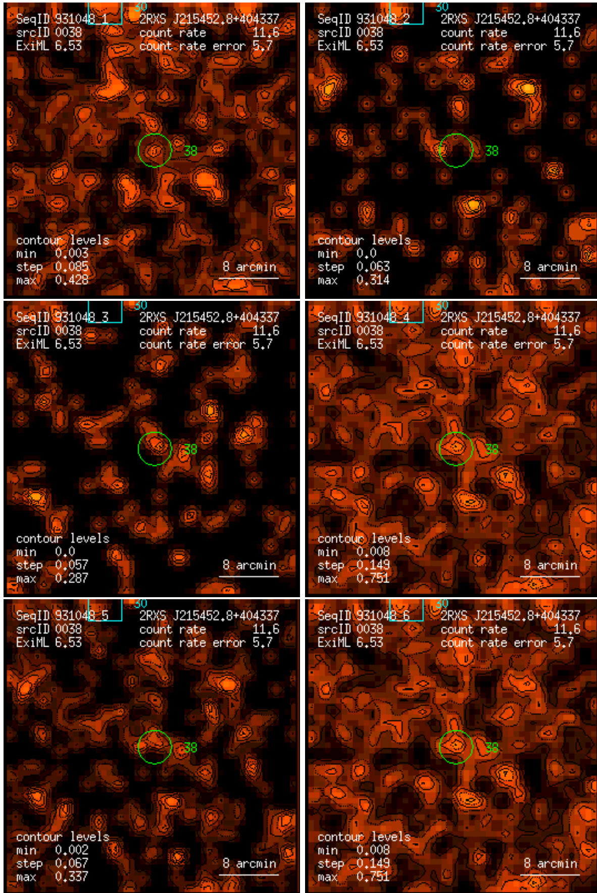
Figure 38: RASS 931048: detection 0038: band rate images, Gaussian filter: (1) PSPC channels 11 – 41, (2) 52 – 90, (3) 91 – 201, (4) 11 – 235, (5) 52 – 201, (6) 11 – 201. Broad band rates in counts/ks. Band rate contour levels in counts/ks/arcmin 2 .
