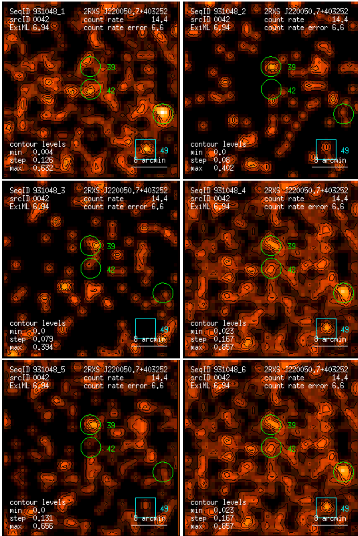
Figure 42: RASS 931048: detection 0042: band rate images, Gaussian filter: (1) PSPC channels 11 – 41, (2) 52 – 90, (3) 91 – 201, (4) 11 – 235, (5) 52 – 201, (6) 11 – 201. Broad band rates in counts/ks. Band rate contour levels in counts/ks/arcmin 2 .
