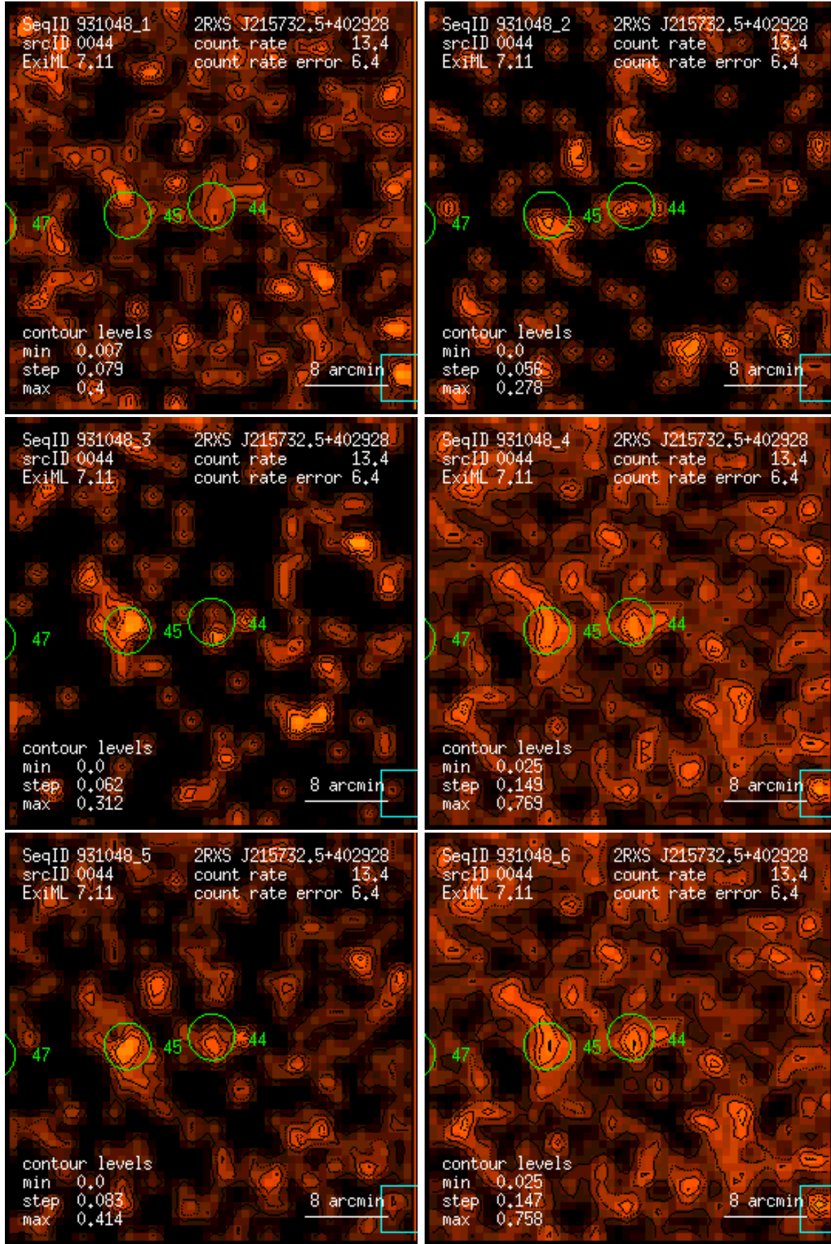
Figure 44: RASS 931048: detection 0044: band rate images, Gaussian filter: (1) PSPC channels 11 – 41, (2) 52 – 90, (3) 91 – 201, (4) 11 – 235, (5) 52 – 201, (6) 11 – 201. Broad band rates in counts/ks. Band rate contour levels in counts/ks/arcmin 2 .
