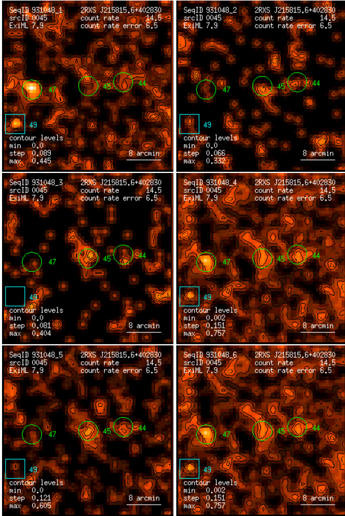
Figure 45: RASS 931048: detection 0045: band rate images, Gaussian filter: (1) PSPC channels 11 – 41, (2) 52 – 90, (3) 91 – 201, (4) 11 – 235, (5) 52 – 201, (6) 11 – 201. Broad band rates in counts/ks. Band rate contour levels in counts/ks/arcmin 2 .
