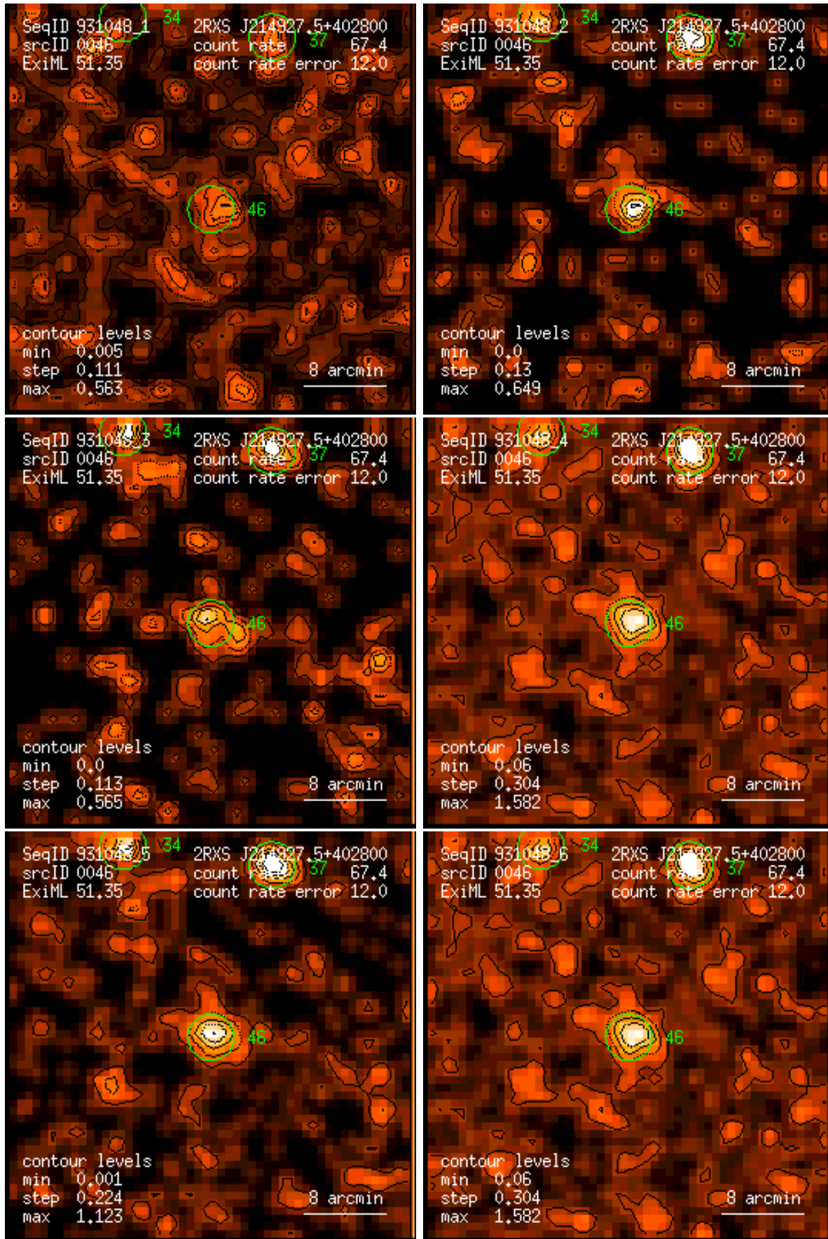
Figure 46: RASS 931048: detection 0046: band rate images, Gaussian filter: (1) PSPC channels 11 – 41, (2) 52 – 90, (3) 91 – 201, (4) 11 – 235, (5) 52 – 201, (6) 11 – 201. Broad band rates in counts/ks. Band rate contour levels in counts/ks/arcmin 2 .
