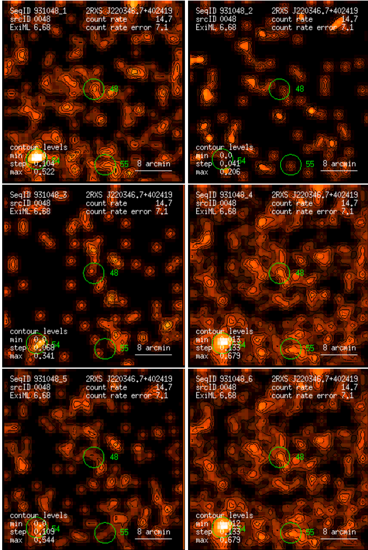
Figure 48: RASS 931048: detection 0048: band rate images, Gaussian filter: (1) PSPC channels 11 – 41, (2) 52 – 90, (3) 91 – 201, (4) 11 – 235, (5) 52 – 201, (6) 11 – 201. Broad band rates in counts/ks. Band rate contour levels in counts/ks/arcmin 2 .
