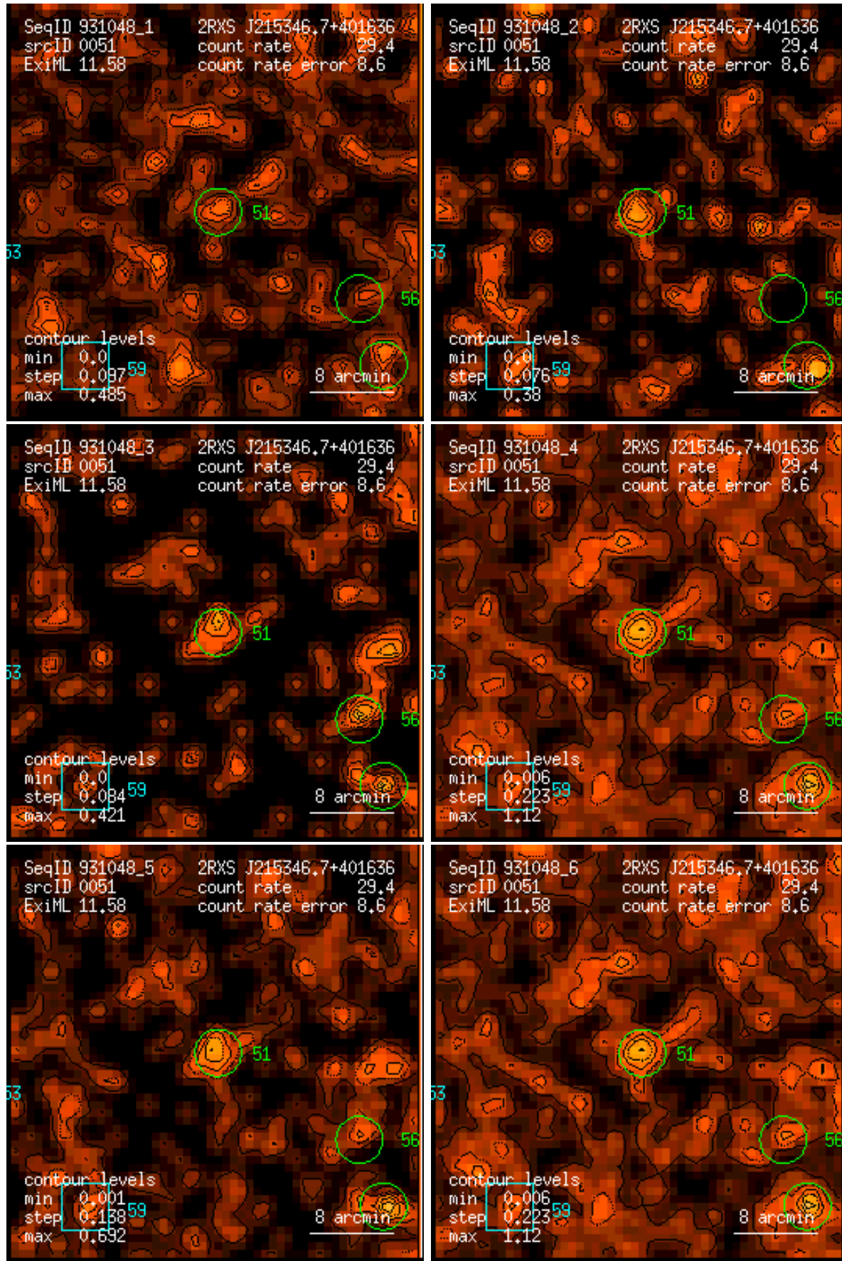
Figure 51: RASS 931048: detection 0051: band rate images, Gaussian filter: (1) PSPC channels 11 – 41, (2) 52 – 90, (3) 91 – 201, (4) 11 – 235, (5) 52 – 201, (6) 11 – 201. Broad band rates in counts/ks. Band rate contour levels in counts/ks/arcmin 2 .
