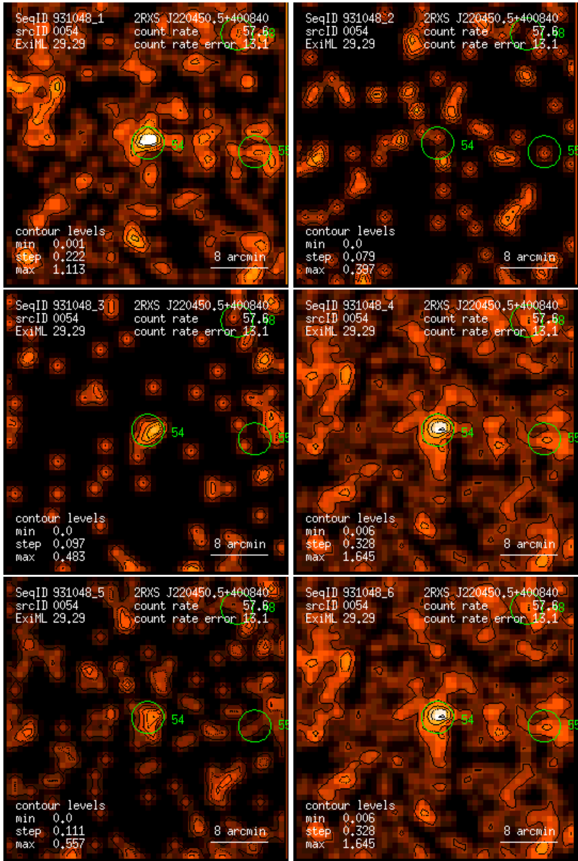
Figure 54: RASS 931048: detection 0054: band rate images, Gaussian filter: (1) PSPC channels 11 – 41, (2) 52 – 90, (3) 91 – 201, (4) 11 – 235, (5) 52 – 201, (6) 11 – 201. Broad band rates in counts/ks. Band rate contour levels in counts/ks/arcmin 2 .
