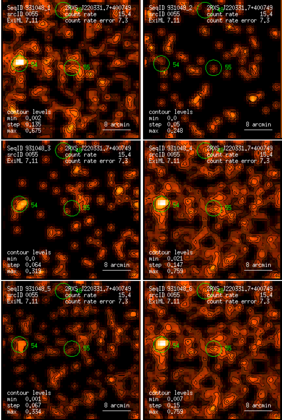
Figure 55: RASS 931048: detection 0055: band rate images, Gaussian filter: (1) PSPC channels 11 – 41, (2) 52 – 90, (3) 91 – 201, (4) 11 – 235, (5) 52 – 201, (6) 11 – 201. Broad band rates in counts/ks. Band rate contour levels in counts/ks/arcmin 2 .
