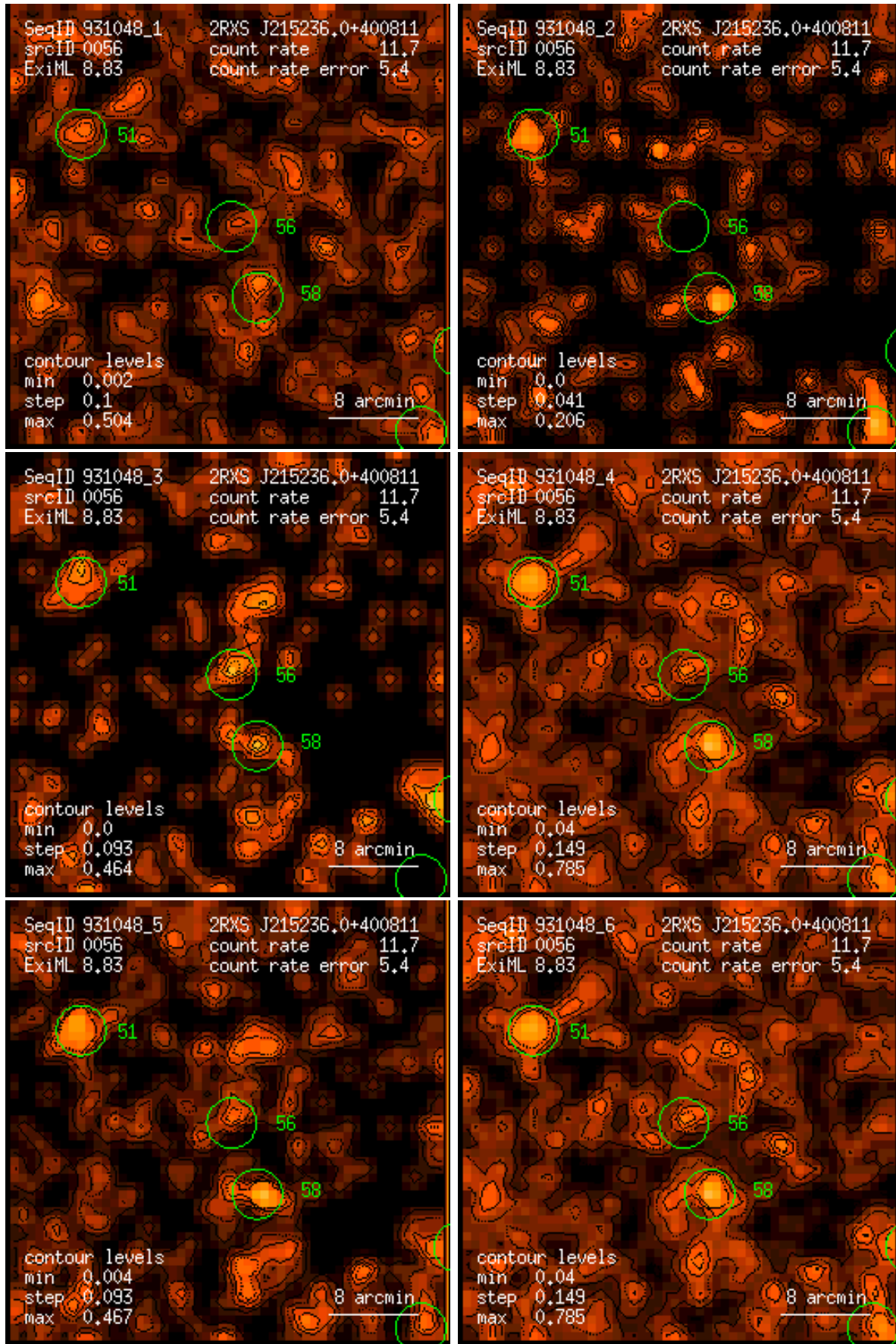
Figure 56: RASS 931048: detection 0056: band rate images, Gaussian filter: (1) PSPC channels 11 – 41, (2) 52 – 90, (3) 91 – 201, (4) 11 – 235, (5) 52 – 201, (6) 11 – 201. Broad band rates in counts/ks. Band rate contour levels in counts/ks/arcmin 2 .
