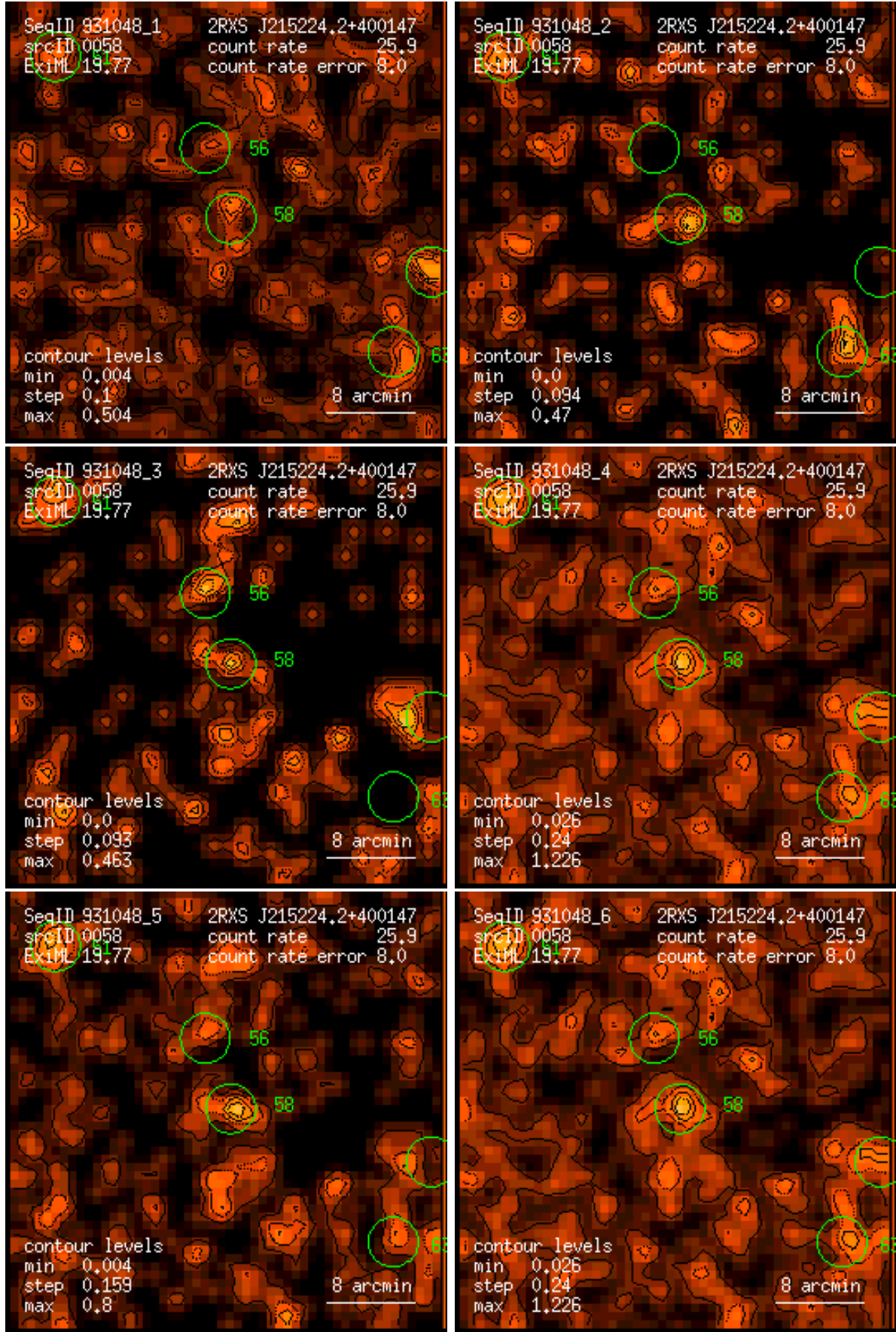
Figure 58: RASS 931048: detection 0058: band rate images, Gaussian filter: (1) PSPC channels 11 – 41, (2) 52 – 90, (3) 91 – 201, (4) 11 – 235, (5) 52 – 201, (6) 11 – 201. Broad band rates in counts/ks. Band rate contour levels in counts/ks/arcmin 2 .
