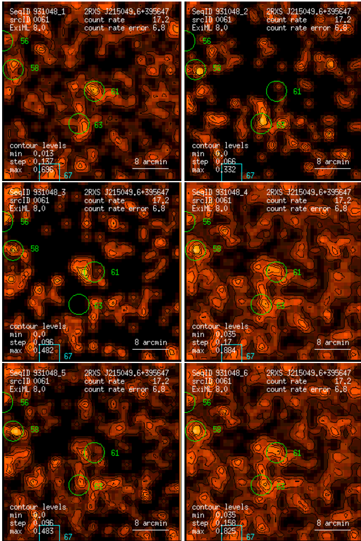
Figure 61: RASS 931048: detection 0061: band rate images, Gaussian filter: (1) PSPC channels 11 – 41, (2) 52 – 90, (3) 91 – 201, (4) 11 – 235, (5) 52 – 201, (6) 11 – 201. Broad band rates in counts/ks. Band rate contour levels in counts/ks/arcmin 2 .
