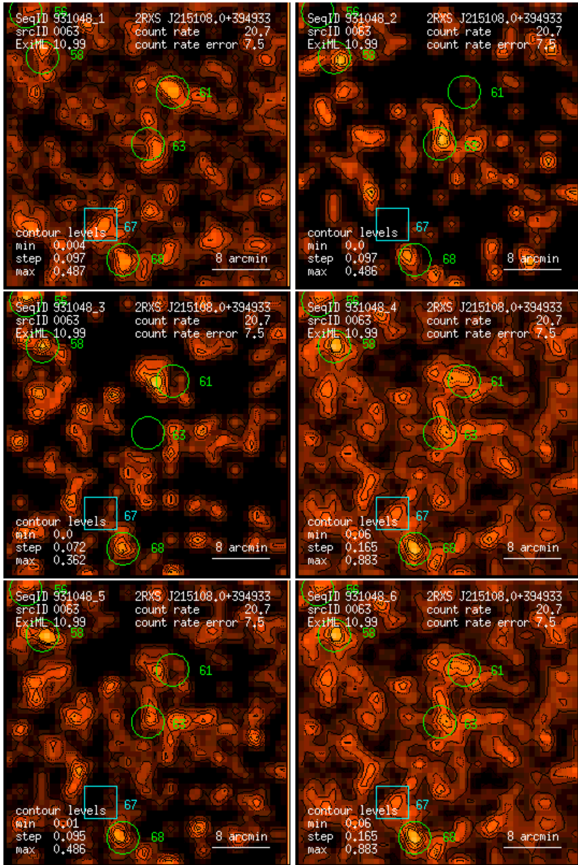
Figure 63: RASS 931048: detection 0063: band rate images, Gaussian filter: (1) PSPC channels 11 – 41, (2) 52 – 90, (3) 91 – 201, (4) 11 – 235, (5) 52 – 201, (6) 11 – 201. Broad band rates in counts/ks. Band rate contour levels in counts/ks/arcmin 2 .
