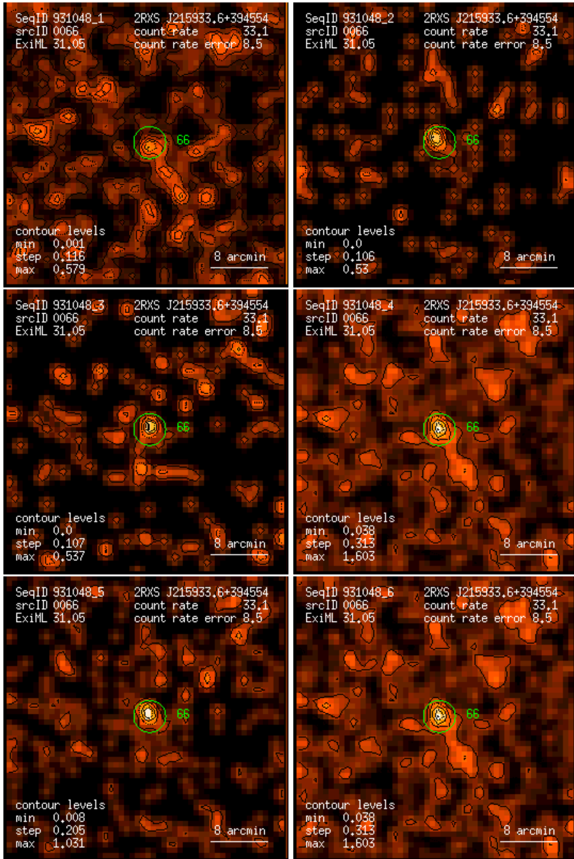
Figure 66: RASS 931048: detection 0066: band rate images, Gaussian filter: (1) PSPC channels 11 – 41, (2) 52 – 90, (3) 91 – 201, (4) 11 – 235, (5) 52 – 201, (6) 11 – 201. Broad band rates in counts/ks. Band rate contour levels in counts/ks/arcmin 2 .
