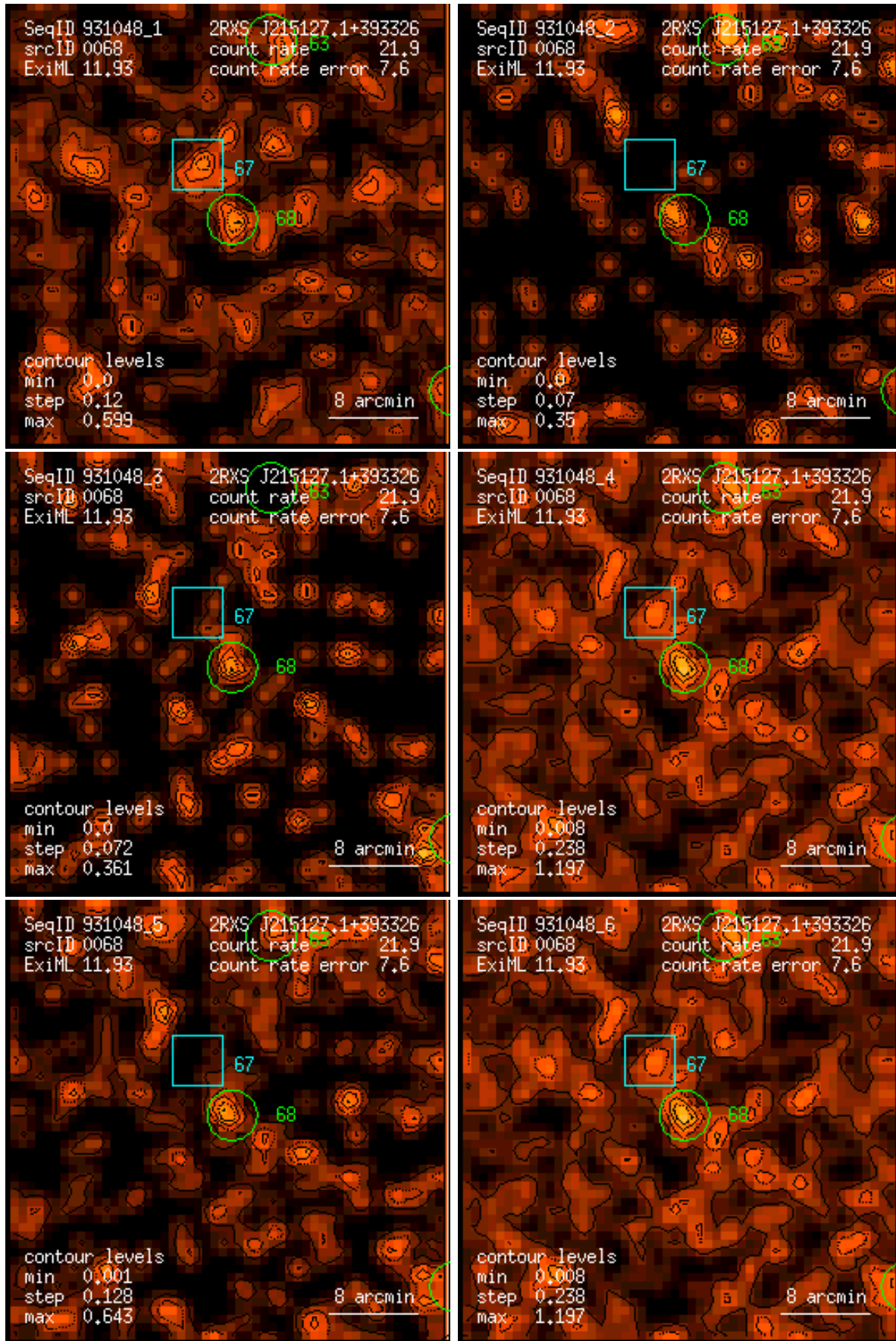
Figure 68: RASS 931048: detection 0068: band rate images, Gaussian filter: (1) PSPC channels 11 – 41, (2) 52 – 90, (3) 91 – 201, (4) 11 – 235, (5) 52 – 201, (6) 11 – 201. Broad band rates in counts/ks. Band rate contour levels in counts/ks/arcmin 2 .
