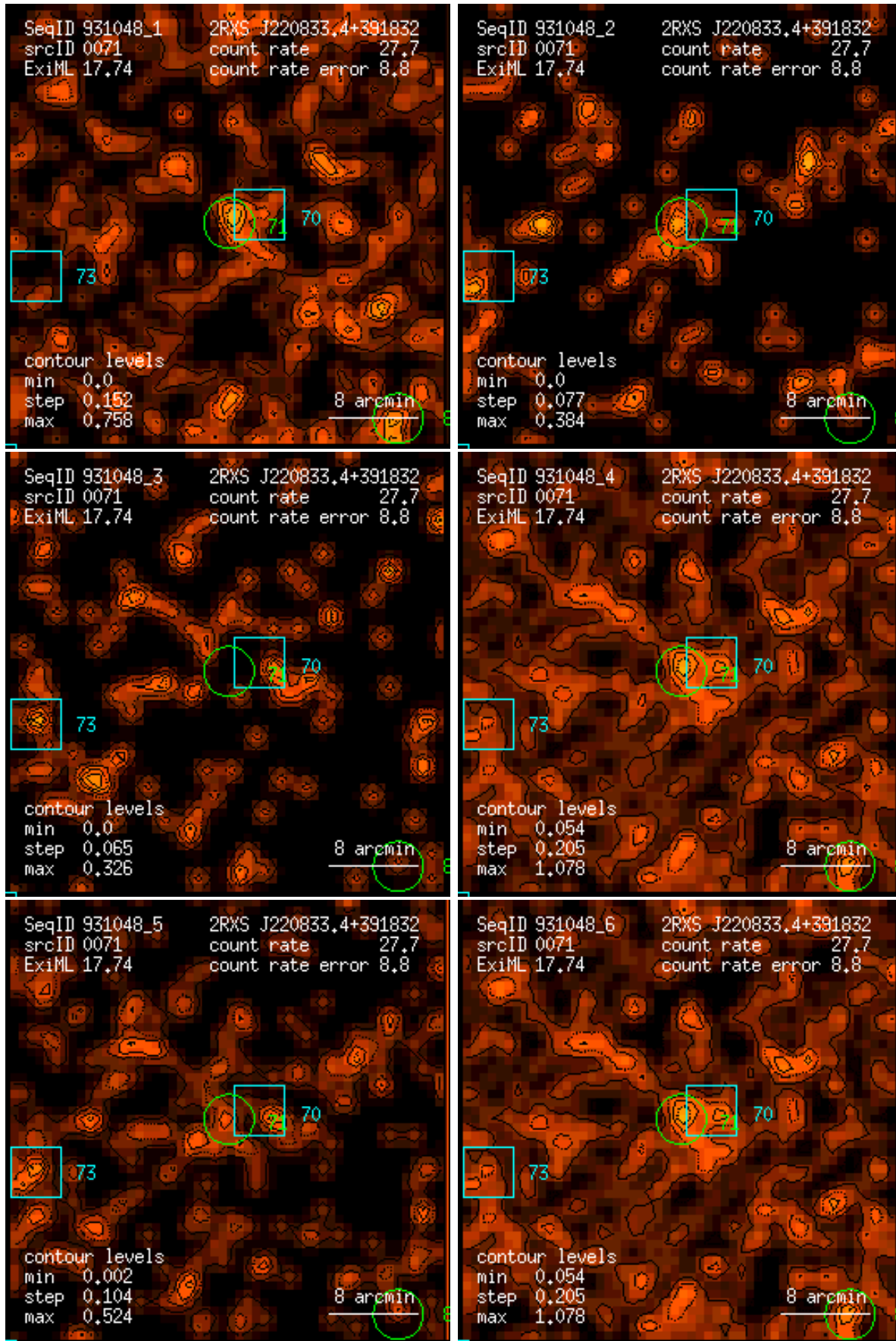
Figure 71: RASS 931048: detection 0071: band rate images, Gaussian filter: (1) PSPC channels 11 – 41, (2) 52 – 90, (3) 91 – 201, (4) 11 – 235, (5) 52 – 201, (6) 11 – 201. Broad band rates in counts/ks. Band rate contour levels in counts/ks/arcmin 2 .
