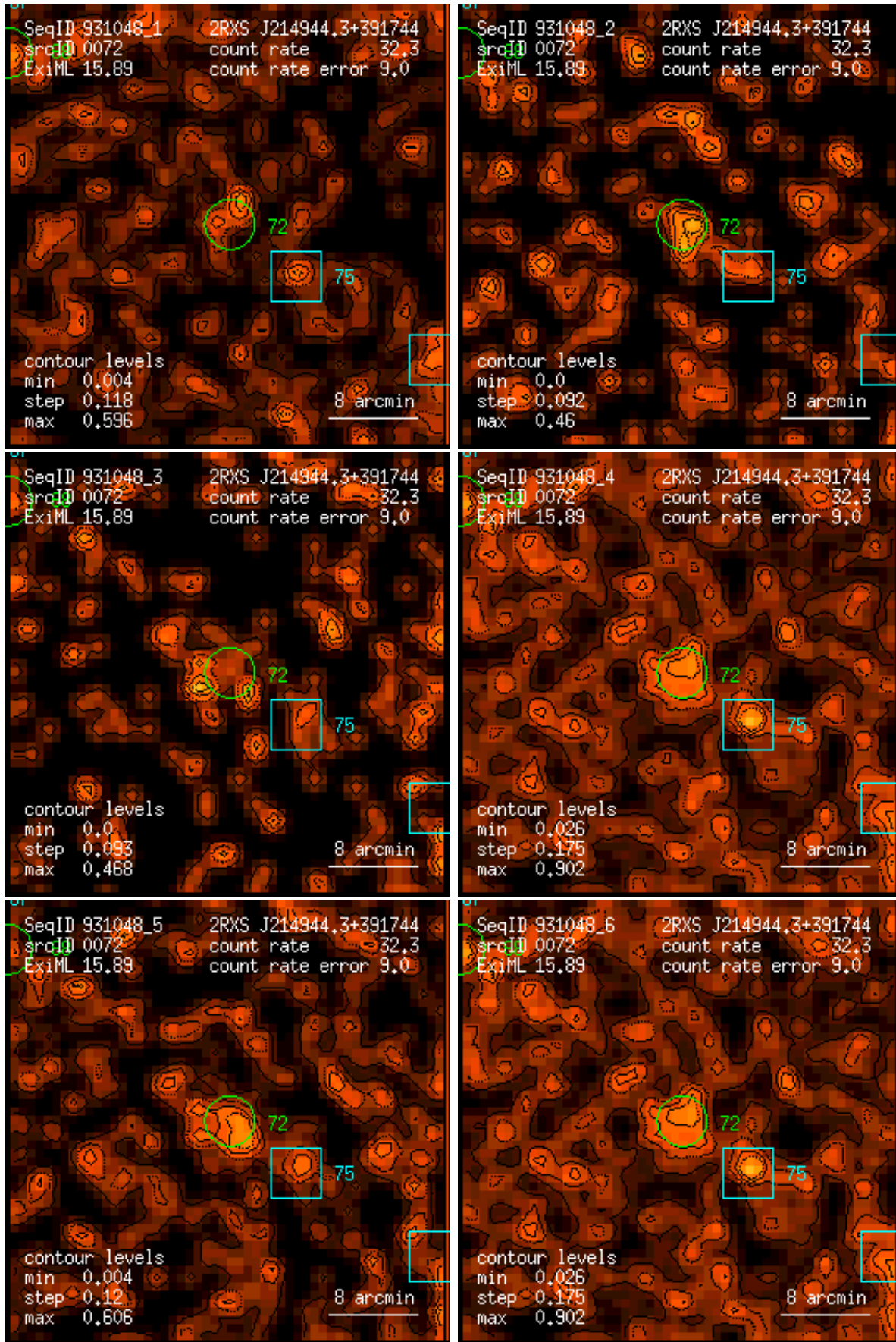
Figure 72: RASS 931048: detection 0072: band rate images, Gaussian filter: (1) PSPC channels 11 – 41, (2) 52 – 90, (3) 91 – 201, (4) 11 – 235, (5) 52 – 201, (6) 11 – 201. Broad band rates in counts/ks. Band rate contour levels in counts/ks/arcmin 2 .
