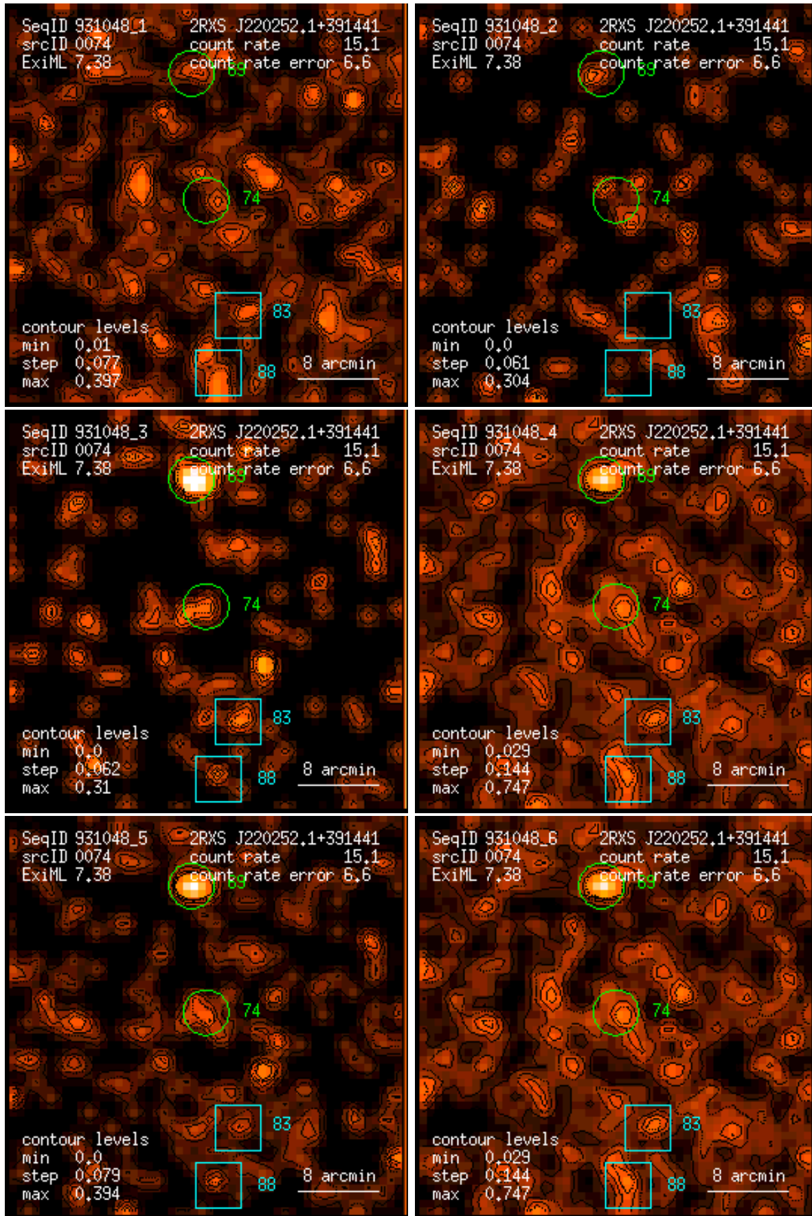
Figure 74: RASS 931048: detection 0074: band rate images, Gaussian filter: (1) PSPC channels 11 – 41, (2) 52 – 90, (3) 91 – 201, (4) 11 – 235, (5) 52 – 201, (6) 11 – 201. Broad band rates in counts/ks. Band rate contour levels in counts/ks/arcmin 2 .
