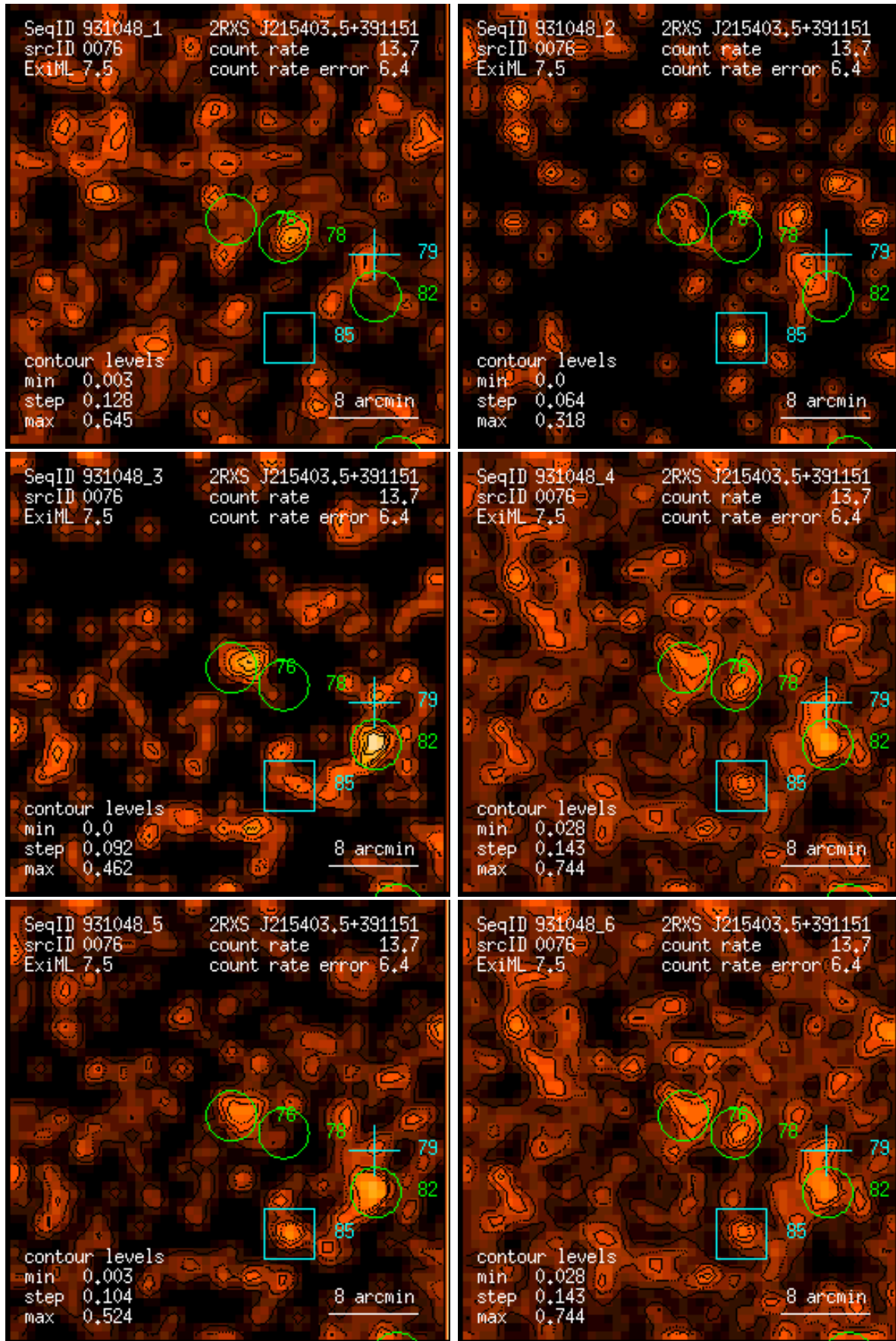
Figure 76: RASS 931048: detection 0076: band rate images, Gaussian filter: (1) PSPC channels 11 – 41, (2) 52 – 90, (3) 91 – 201, (4) 11 – 235, (5) 52 – 201, (6) 11 – 201. Broad band rates in counts/ks. Band rate contour levels in counts/ks/arcmin 2 .
