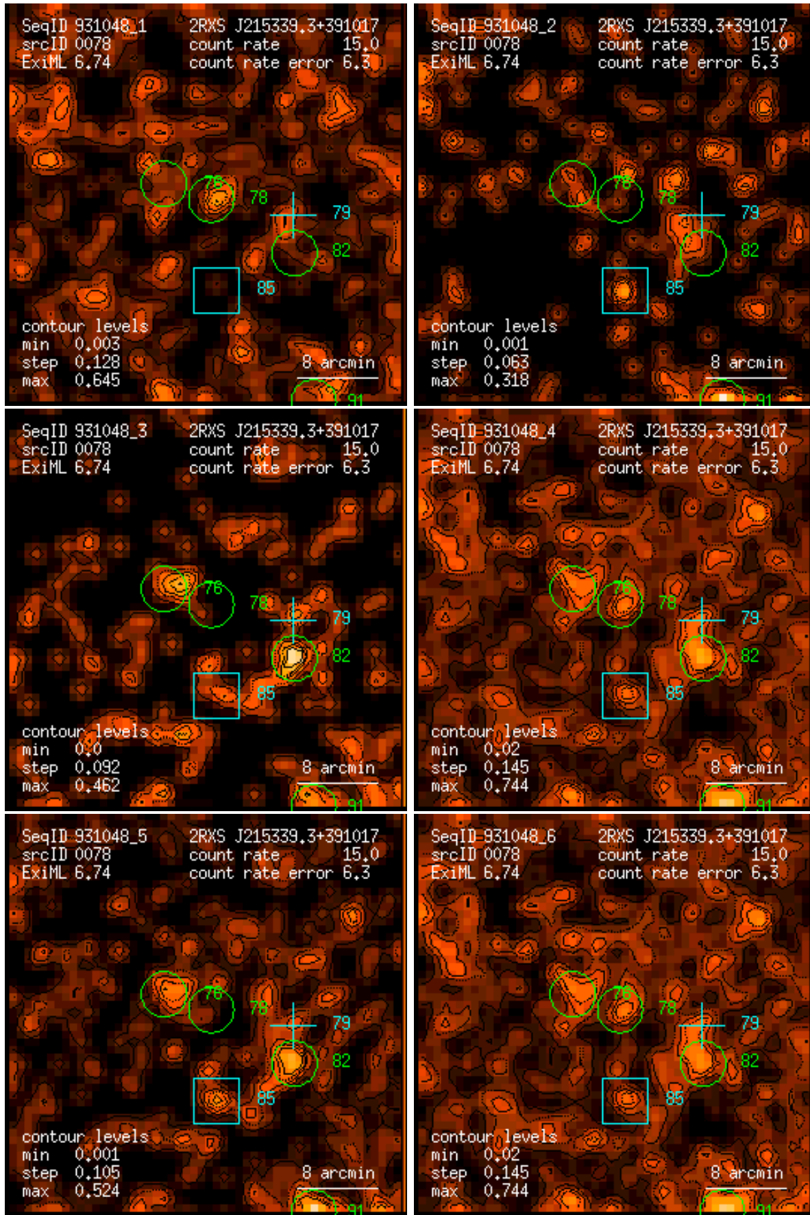
Figure 78: RASS 931048: detection 0078: band rate images, Gaussian filter: (1) PSPC channels 11 – 41, (2) 52 – 90, (3) 91 – 201, (4) 11 – 235, (5) 52 – 201, (6) 11 – 201. Broad band rates in counts/ks. Band rate contour levels in counts/ks/arcmin 2 .
