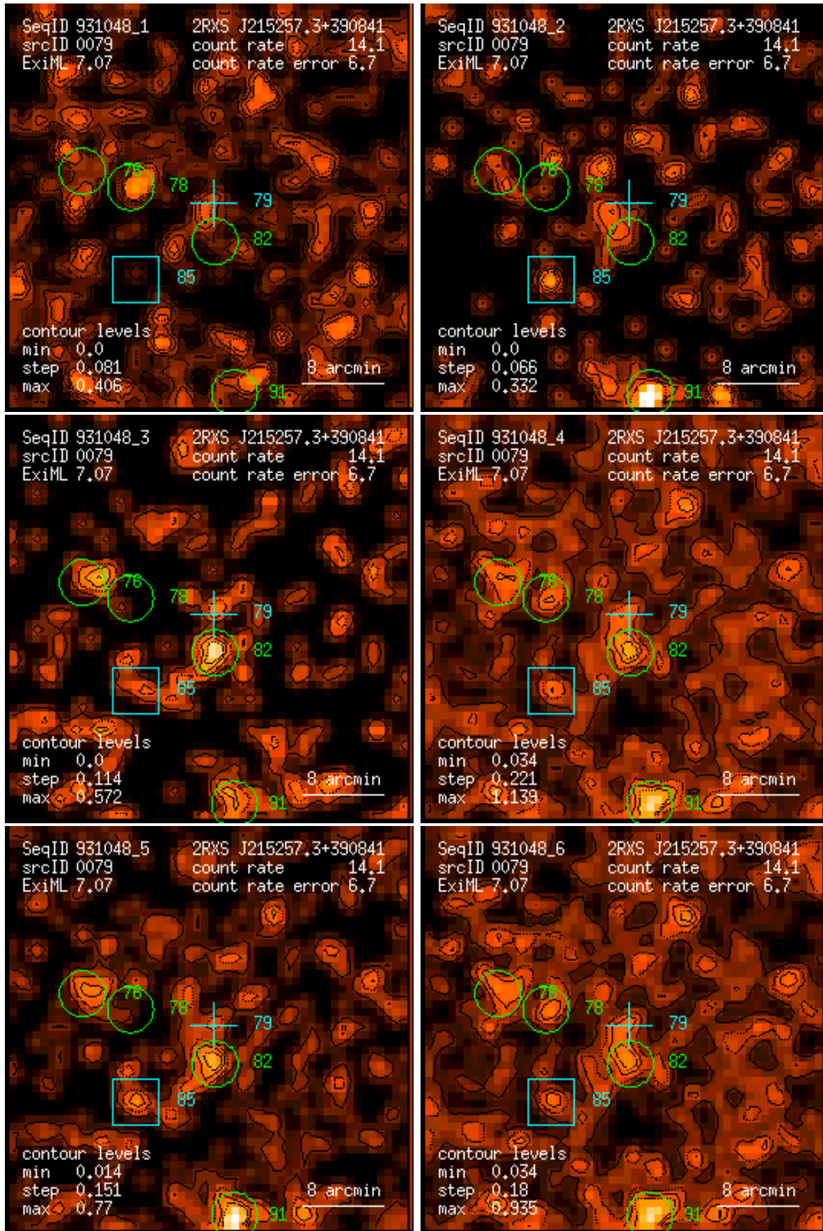
Figure 79: RASS 931048: detection 0079: band rate images, Gaussian filter: (1) PSPC channels 11 – 41, (2) 52 – 90, (3) 91 – 201, (4) 11 – 235, (5) 52 – 201, (6) 11 – 201. Broad band rates in counts/ks. Band rate contour levels in counts/ks/arcmin 2 .
