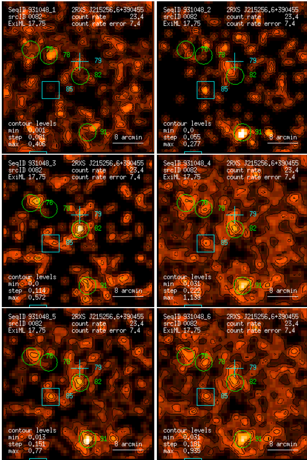
Figure 82: RASS 931048: detection 0082: band rate images, Gaussian filter: (1) PSPC channels 11 – 41, (2) 52 – 90, (3) 91 – 201, (4) 11 – 235, (5) 52 – 201, (6) 11 – 201. Broad band rates in counts/ks. Band rate contour levels in counts/ks/arcmin 2 .
