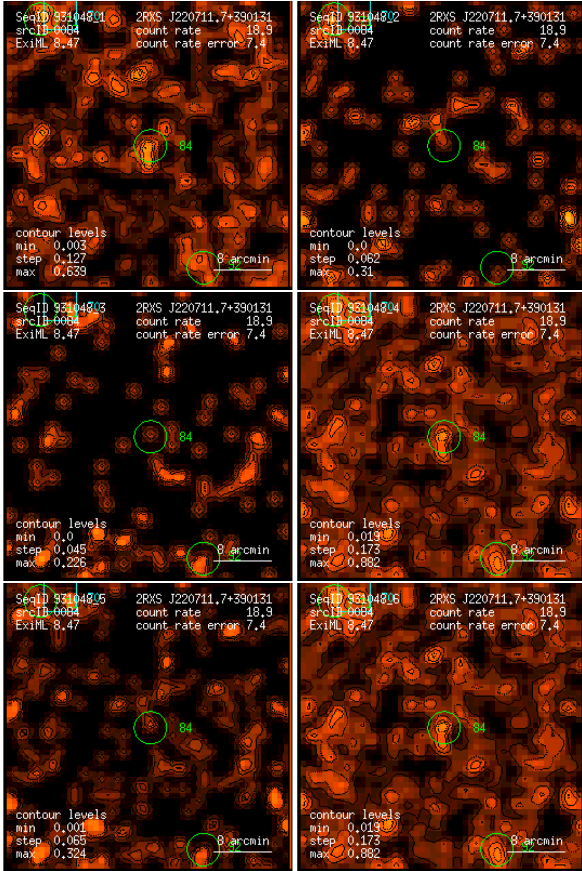
Figure 84: RASS 931048: detection 0084: band rate images, Gaussian filter: (1) PSPC channels 11 – 41, (2) 52 – 90, (3) 91 – 201, (4) 11 – 235, (5) 52 – 201, (6) 11 – 201. Broad band rates in counts/ks. Band rate contour levels in counts/ks/arcmin 2 .
