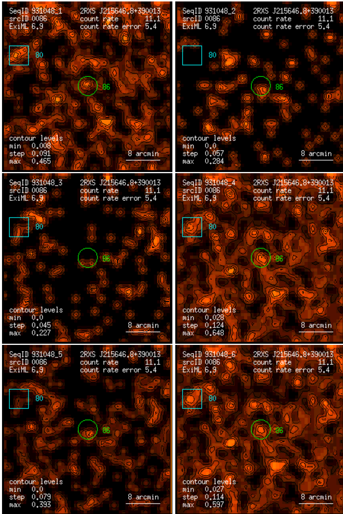
Figure 86: RASS 931048: detection 0086: band rate images, Gaussian filter: (1) PSPC channels 11 – 41, (2) 52 – 90, (3) 91 – 201, (4) 11 – 235, (5) 52 – 201, (6) 11 – 201. Broad band rates in counts/ks. Band rate contour levels in counts/ks/arcmin 2 .
