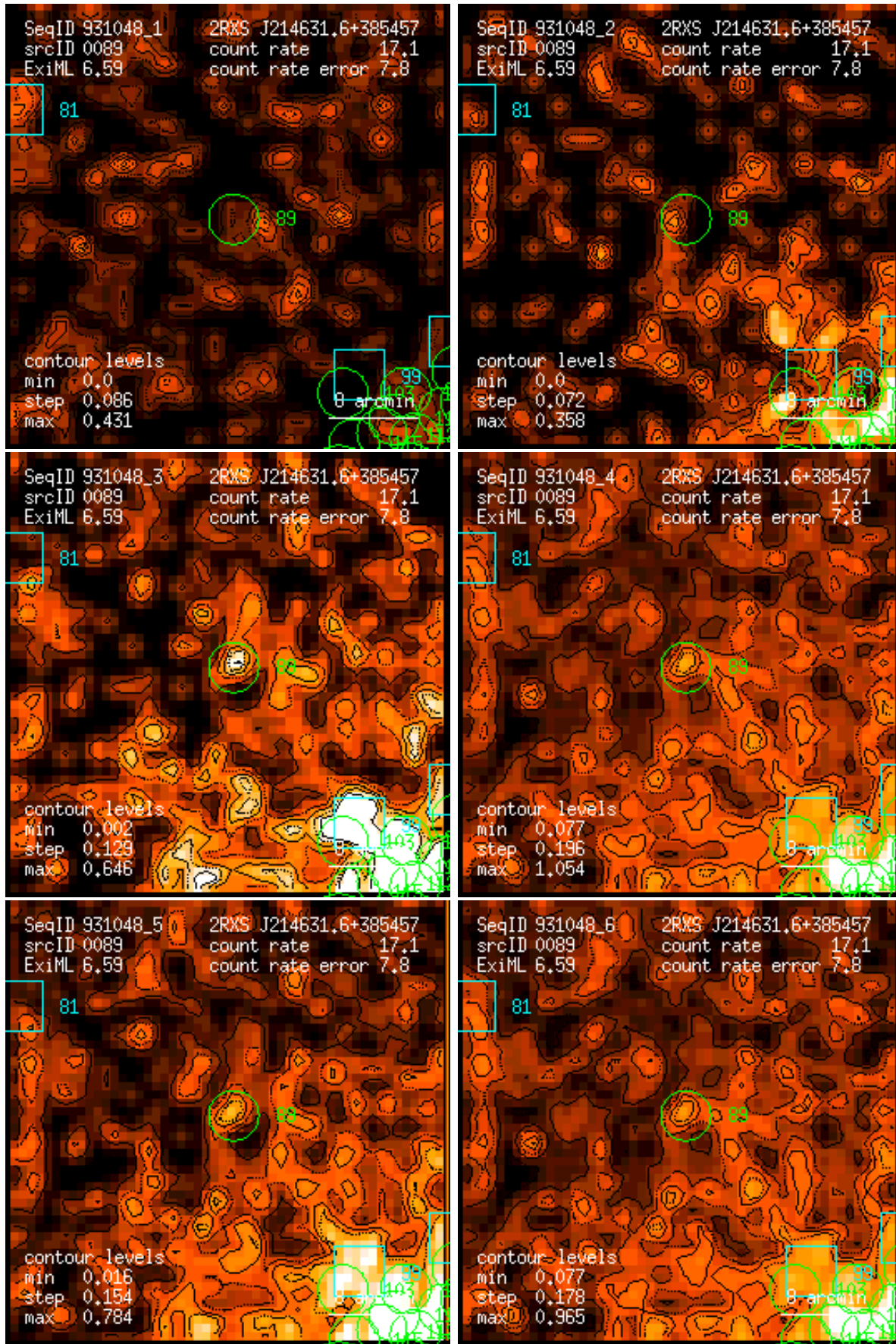
Figure 89: RASS 931048: detection 0089: band rate images, Gaussian filter: (1) PSPC channels 11 – 41, (2) 52 – 90, (3) 91 – 201, (4) 11 – 235, (5) 52 – 201, (6) 11 – 201. Broad band rates in counts/ks. Band rate contour levels in counts/ks/arcmin 2 .
