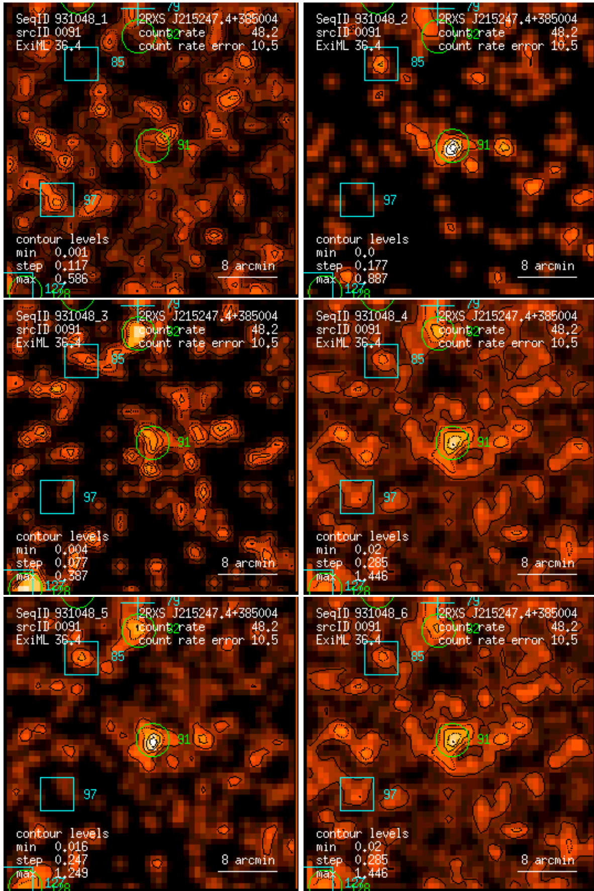
Figure 91: RASS 931048: detection 0091: band rate images, Gaussian filter: (1) PSPC channels 11 – 41, (2) 52 – 90, (3) 91 – 201, (4) 11 – 235, (5) 52 – 201, (6) 11 – 201. Broad band rates in counts/ks. Band rate contour levels in counts/ks/arcmin 2 .
