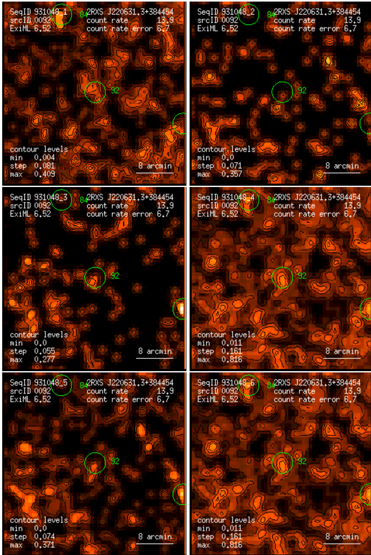
Figure 92: RASS 931048: detection 0092: band rate images, Gaussian filter: (1) PSPC channels 11 – 41, (2) 52 – 90, (3) 91 – 201, (4) 11 – 235, (5) 52 – 201, (6) 11 – 201. Broad band rates in counts/ks. Band rate contour levels in counts/ks/arcmin 2 .
