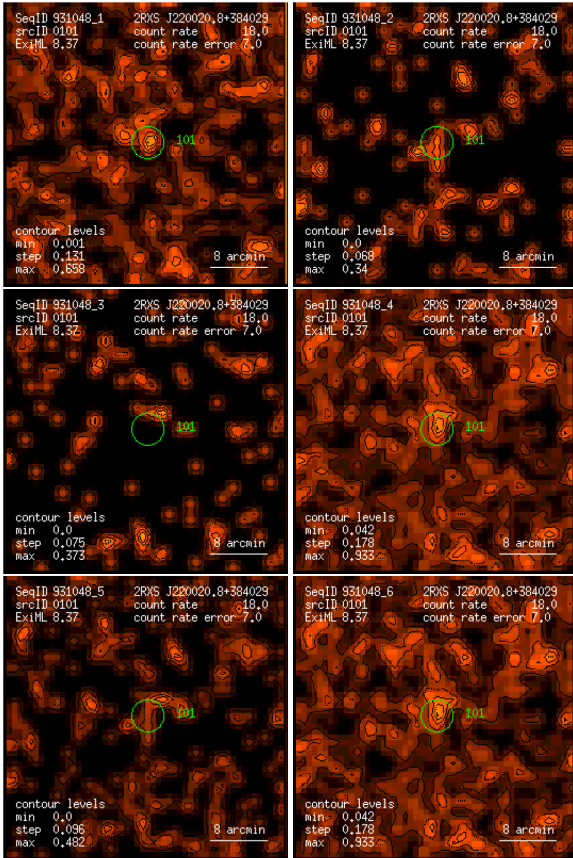
Figure 101: RASS 931048: detection 0101: band rate images, Gaussian filter: (1) PSPC channels 11 – 41, (2) 52 – 90, (3) 91 – 201, (4) 11 – 235, (5) 52 – 201, (6) 11 – 201. Broad band rates in counts/ks. Band rate contour levels in counts/ks/arcmin 2 .
