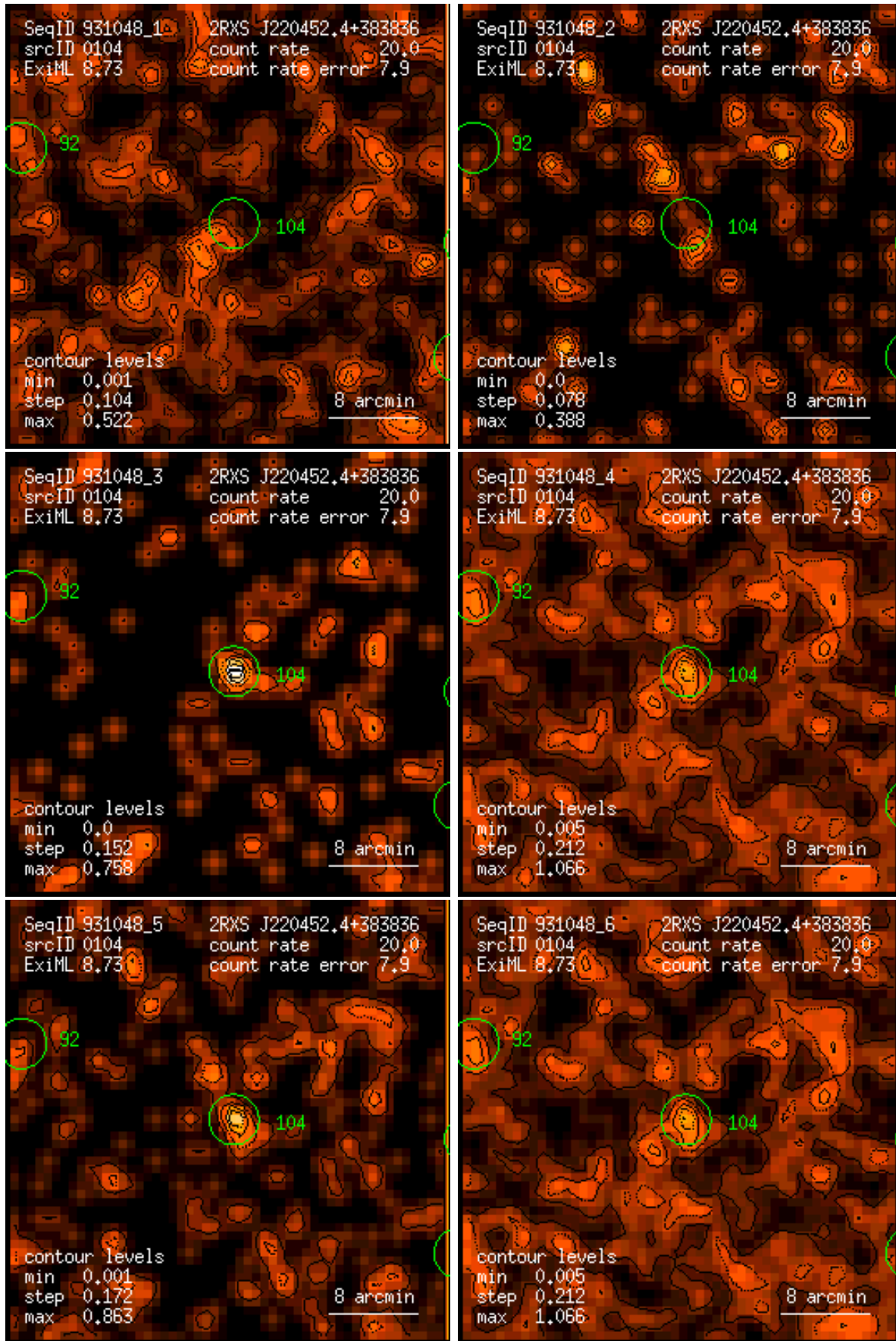
Figure 104: RASS 931048: detection 0104: band rate images, Gaussian filter: (1) PSPC channels 11 – 41, (2) 52 – 90, (3) 91 – 201, (4) 11 – 235, (5) 52 – 201, (6) 11 – 201. Broad band rates in counts/ks. Band rate contour levels in counts/ks/arcmin 2 .
