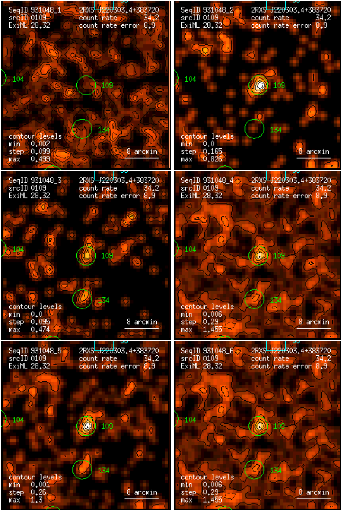
Figure 109: RASS 931048: detection 0109: band rate images, Gaussian filter: (1) PSPC channels 11 – 41, (2) 52 – 90, (3) 91 – 201, (4) 11 – 235, (5) 52 – 201, (6) 11 – 201. Broad band rates in counts/ks. Band rate contour levels in counts/ks/arcmin 2 .
