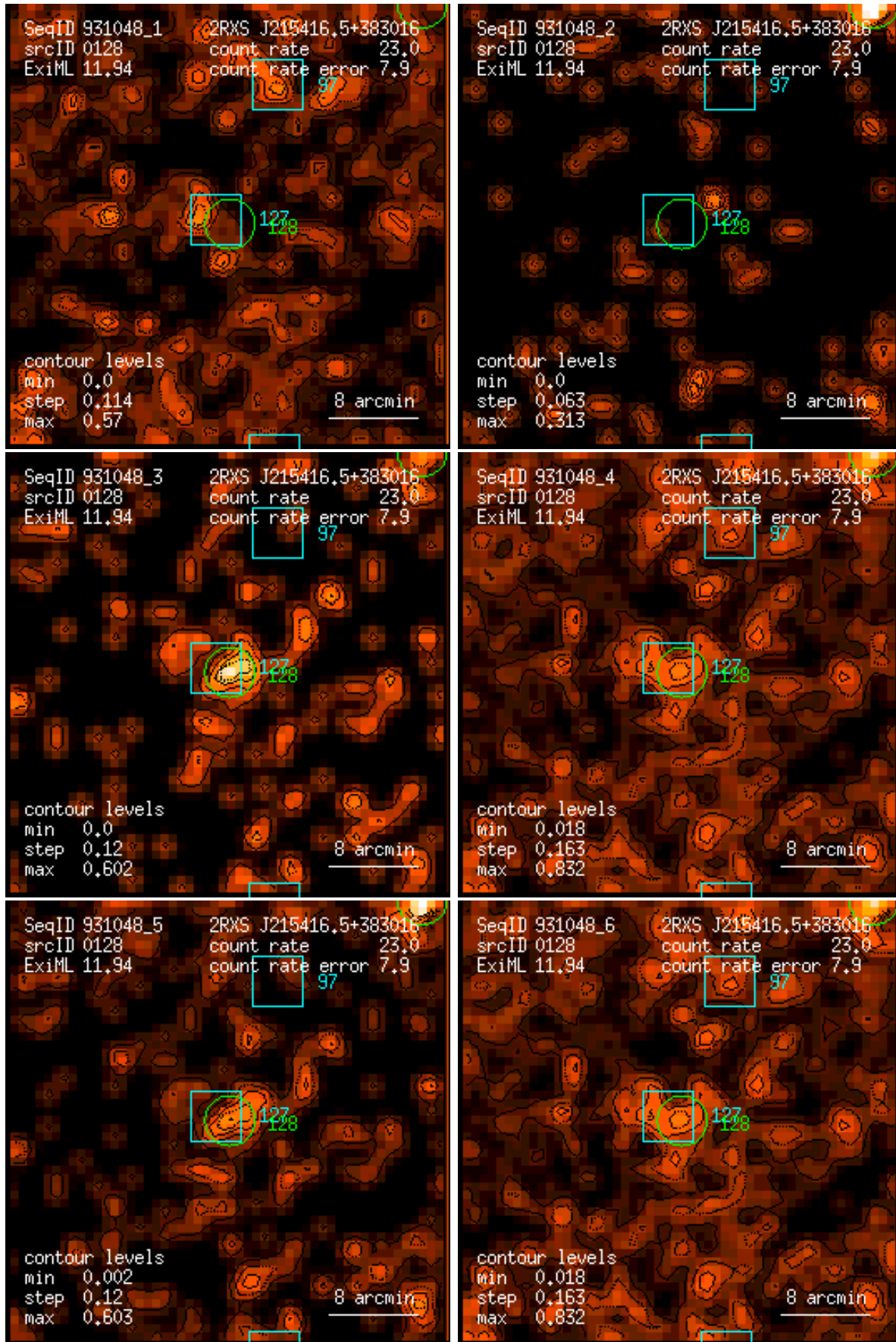
Figure 128: RASS 931048: detection 0128: band rate images, Gaussian filter: (1) PSPC channels 11 – 41, (2) 52 – 90, (3) 91 – 201, (4) 11 – 235, (5) 52 – 201, (6) 11 – 201. Broad band rates in counts/ks. Band rate contour levels in counts/ks/arcmin 2 .
