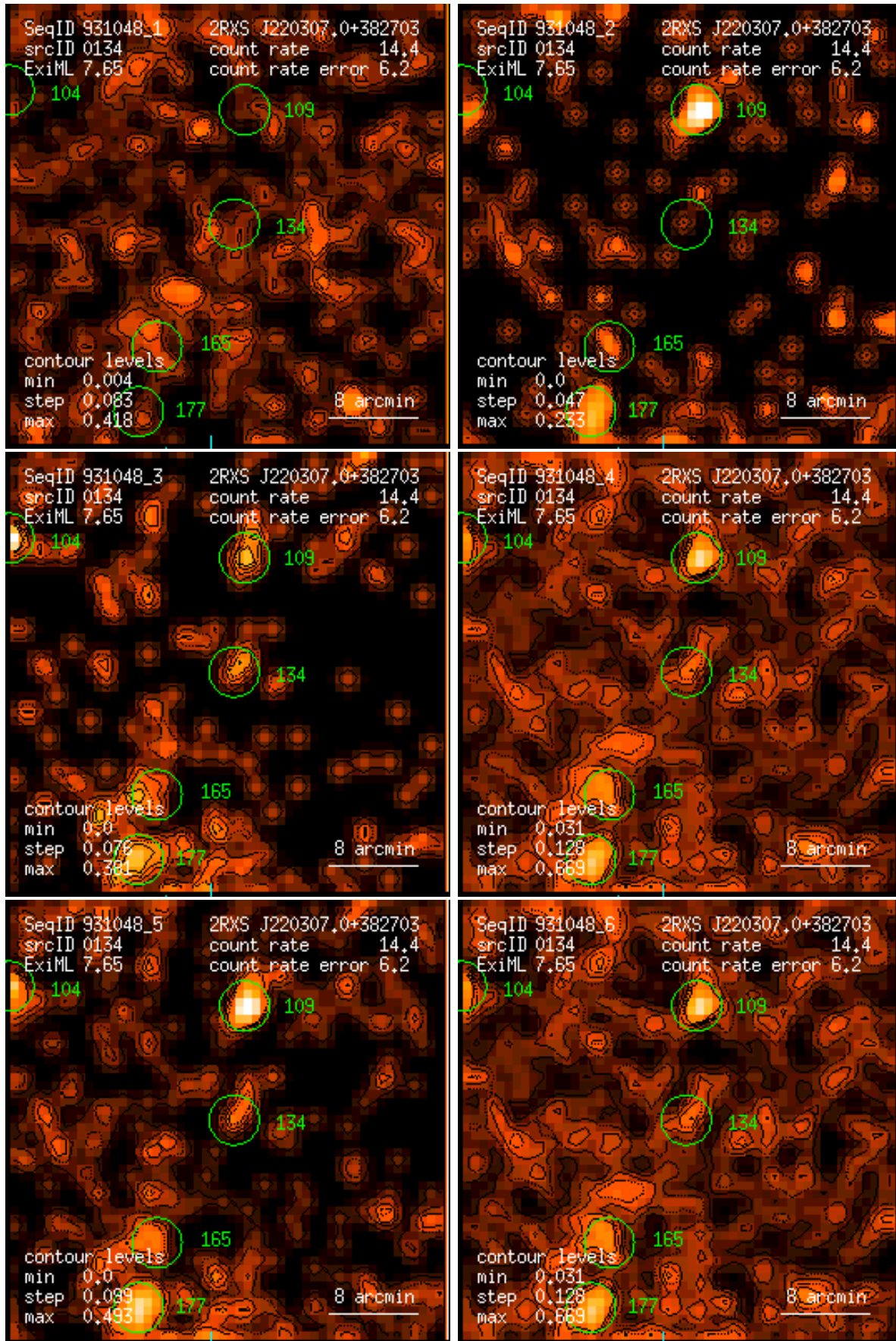
Figure 134: RASS 931048: detection 0134: band rate images, Gaussian filter: (1) PSPC channels 11 – 41, (2) 52 – 90, (3) 91 – 201, (4) 11 – 235, (5) 52 – 201, (6) 11 – 201. Broad band rates in counts/ks. Band rate contour levels in counts/ks/arcmin 2 .
