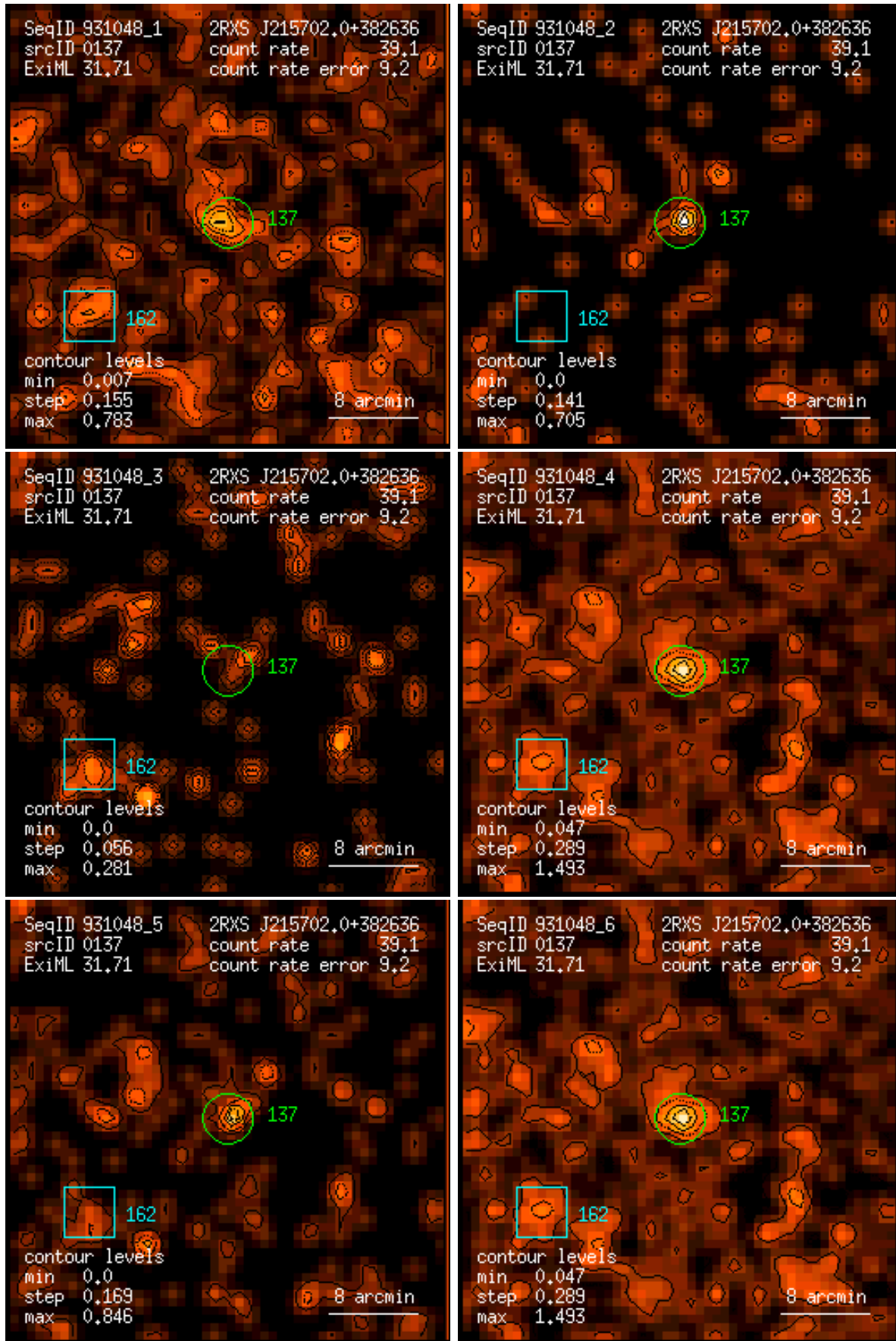
Figure 137: RASS 931048: detection 0137: band rate images, Gaussian filter: (1) PSPC channels 11 – 41, (2) 52 – 90, (3) 91 – 201, (4) 11 – 235, (5) 52 – 201, (6) 11 – 201. Broad band rates in counts/ks. Band rate contour levels in counts/ks/arcmin 2 .
