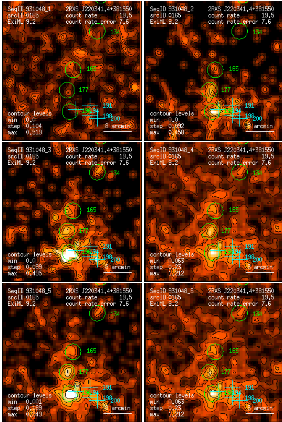
Figure 165: RASS 931048: detection 0165: band rate images, Gaussian filter: (1) PSPC channels 11 – 41, (2) 52 – 90, (3) 91 – 201, (4) 11 – 235, (5) 52 – 201, (6) 11 – 201. Broad band rates in counts/ks. Band rate contour levels in counts/ks/arcmin 2 .
