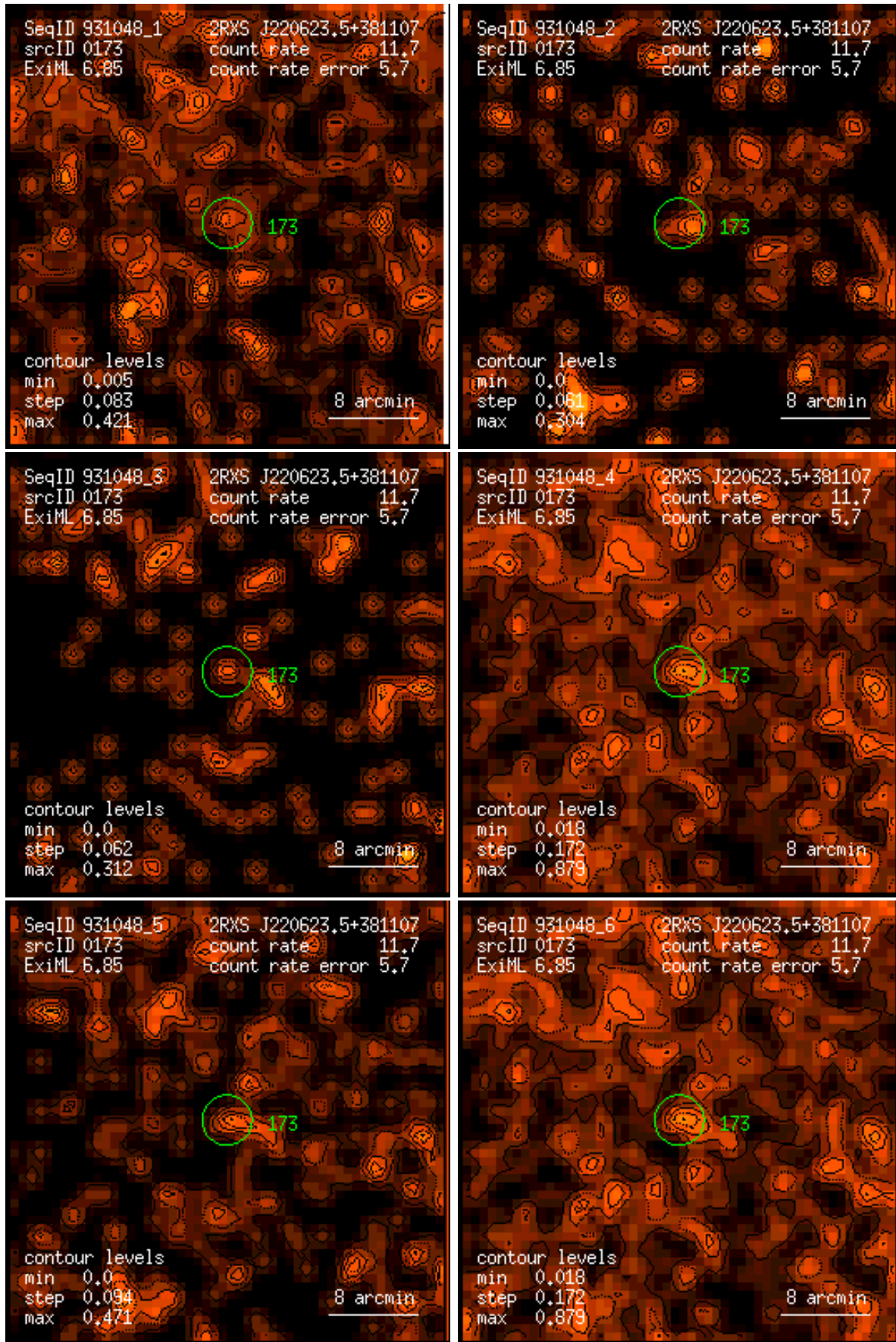
Figure 173: RASS 931048: detection 0173: band rate images, Gaussian filter: (1) PSPC channels 11 – 41, (2) 52 – 90, (3) 91 – 201, (4) 11 – 235, (5) 52 – 201, (6) 11 – 201. Broad band rates in counts/ks. Band rate contour levels in counts/ks/arcmin 2 .
