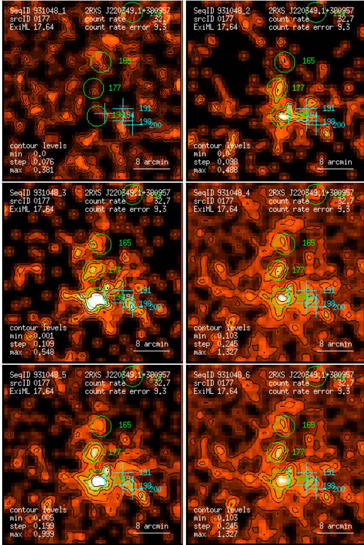
Figure 177: RASS 931048: detection 0177: band rate images, Gaussian filter: (1) PSPC channels 11 – 41, (2) 52 – 90, (3) 91 – 201, (4) 11 – 235, (5) 52 – 201, (6) 11 – 201. Broad band rates in counts/ks. Band rate contour levels in counts/ks/arcmin 2 .
