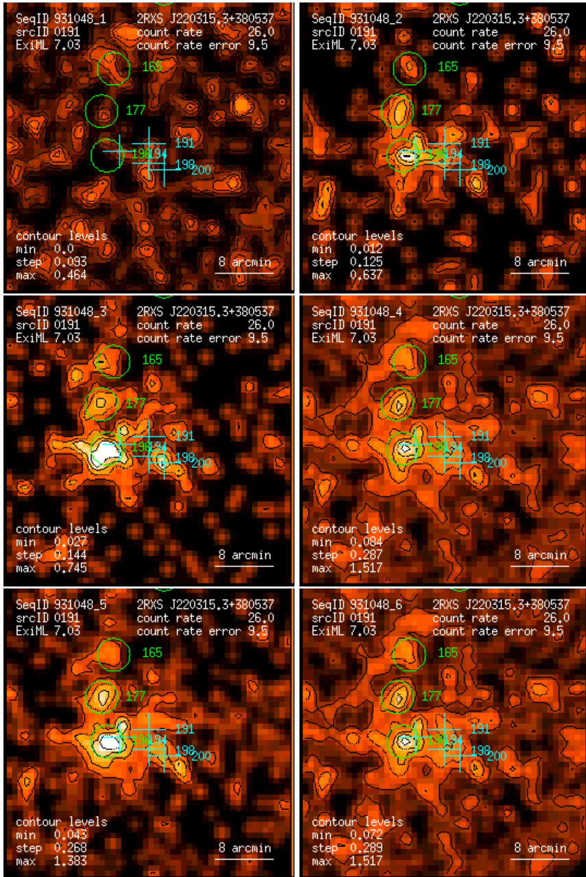
Figure 191: RASS 931048: detection 0191: band rate images, Gaussian filter: (1) PSPC channels 11 – 41, (2) 52 – 90, (3) 91 – 201, (4) 11 – 235, (5) 52 – 201, (6) 11 – 201. Broad band rates in counts/ks. Band rate contour levels in counts/ks/arcmin 2 .
