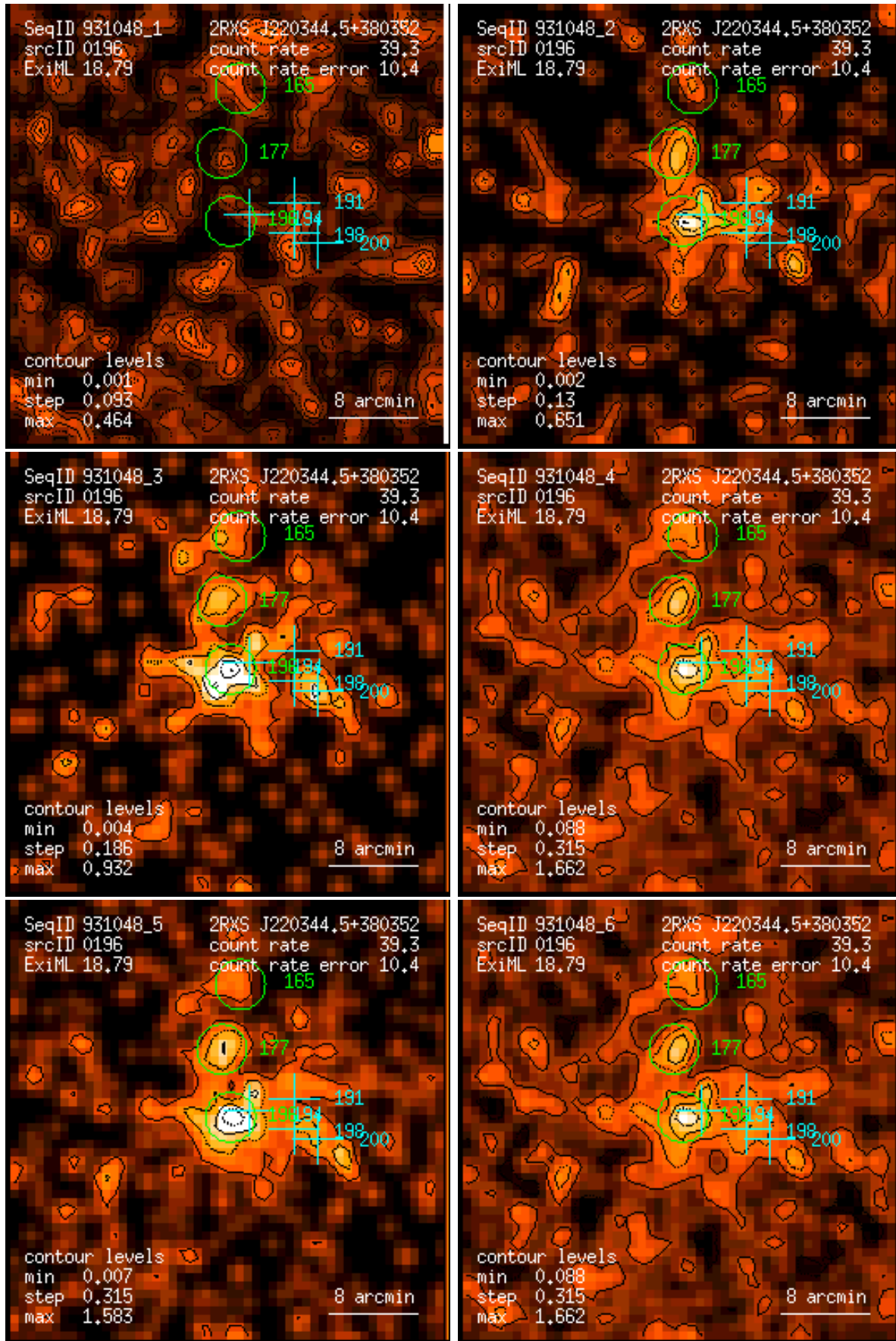
Figure 196: RASS 931048: detection 0196: band rate images, Gaussian filter: (1) PSPC channels 11 – 41, (2) 52 – 90, (3) 91 – 201, (4) 11 – 235, (5) 52 – 201, (6) 11 – 201. Broad band rates in counts/ks. Band rate contour levels in counts/ks/arcmin 2 .
