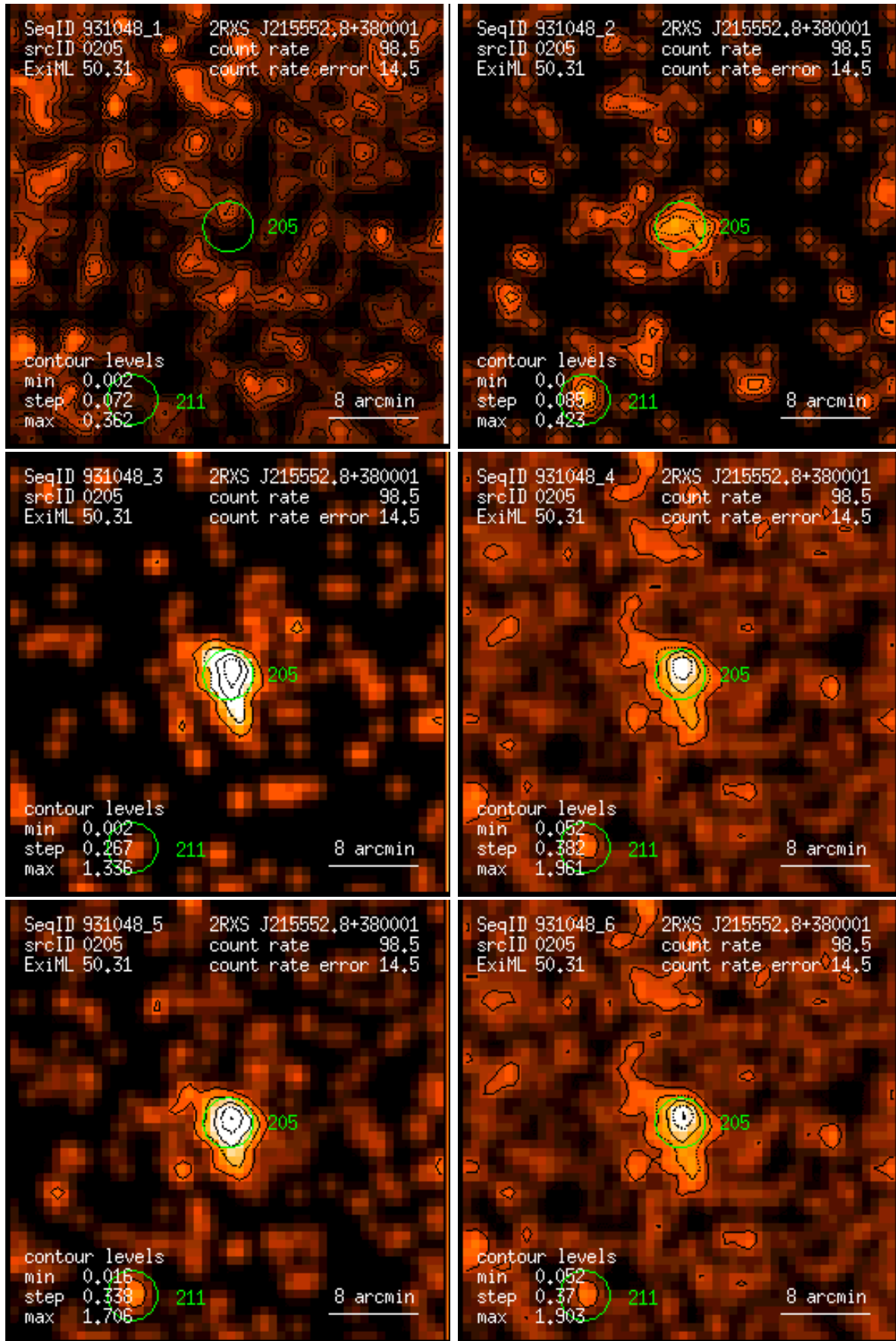
Figure 205: RASS 931048: detection 0205: band rate images, Gaussian filter: (1) PSPC channels 11 – 41, (2) 52 – 90, (3) 91 – 201, (4) 11 – 235, (5) 52 – 201, (6) 11 – 201. Broad band rates in counts/ks. Band rate contour levels in counts/ks/arcmin 2 .
